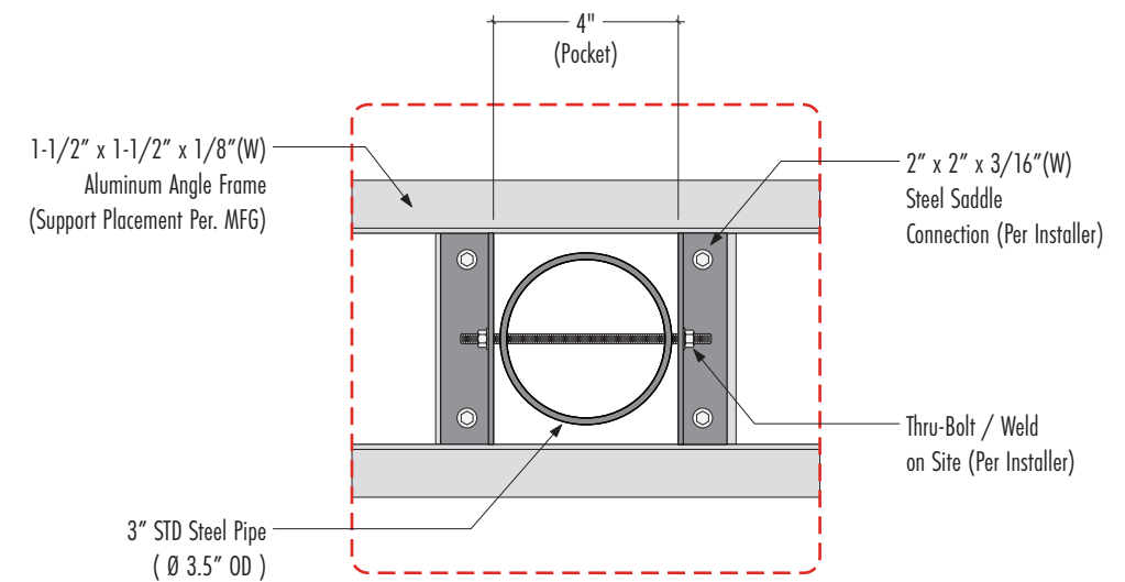
TYP SADDLE DETAIL - TOP VIEW
