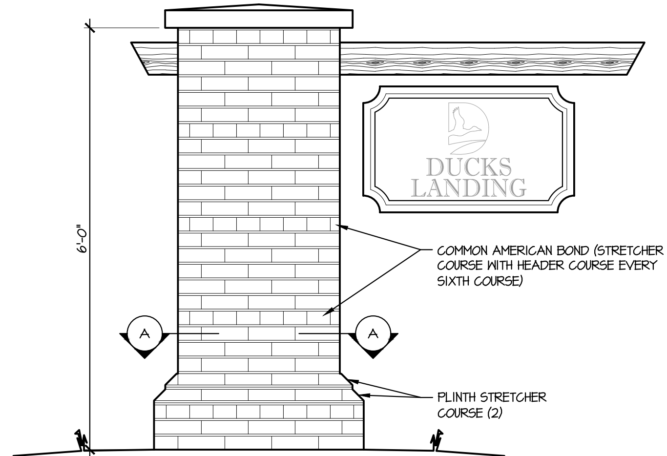
I SIGN & COLUMN ELEVATION 3/4" = 1'-0"
