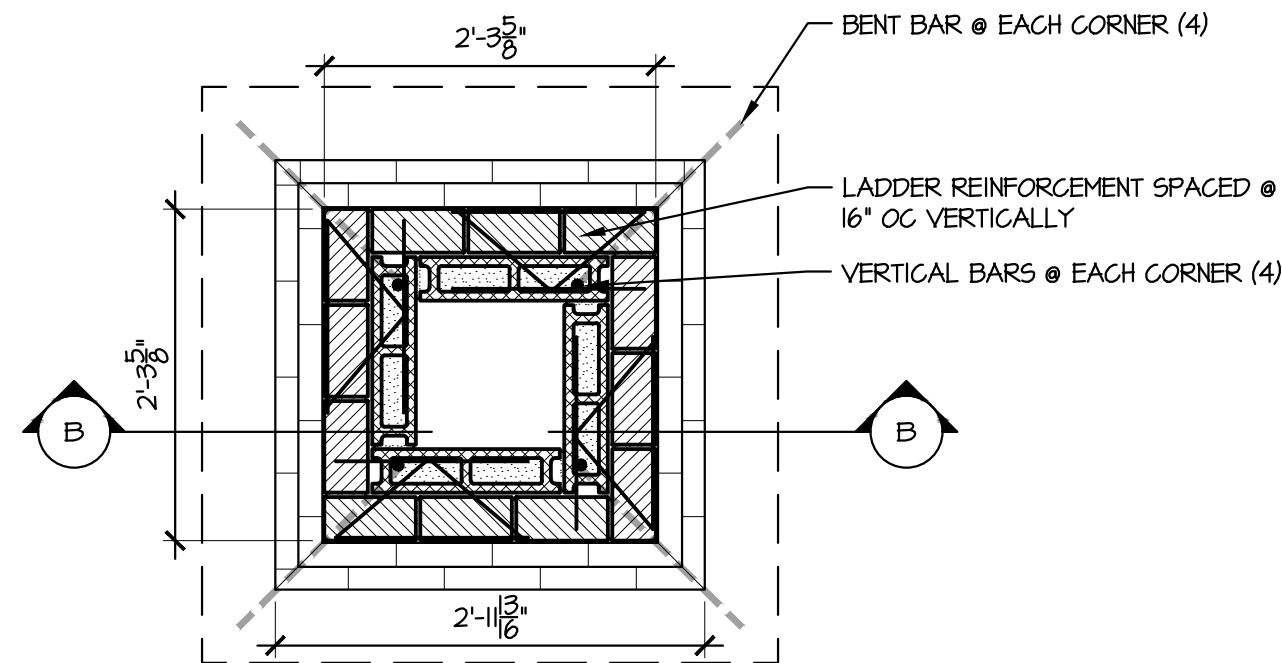
A SIGN & COLUMN PLAN/SECTION 3/4" = 1'-0"
