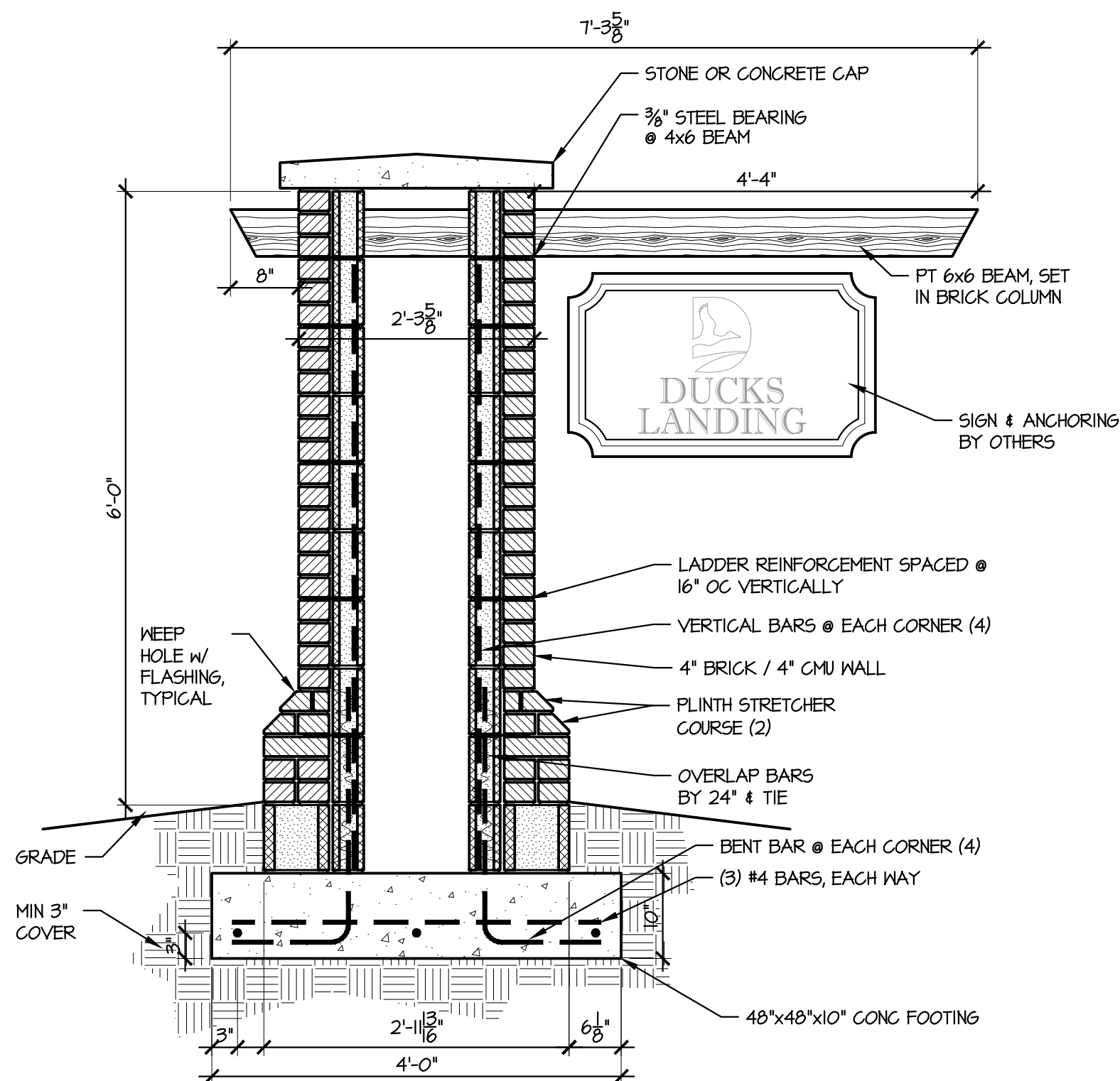
B SIGN & COLUMN VERTICAL SECTION 3/4" = 1'-0"
