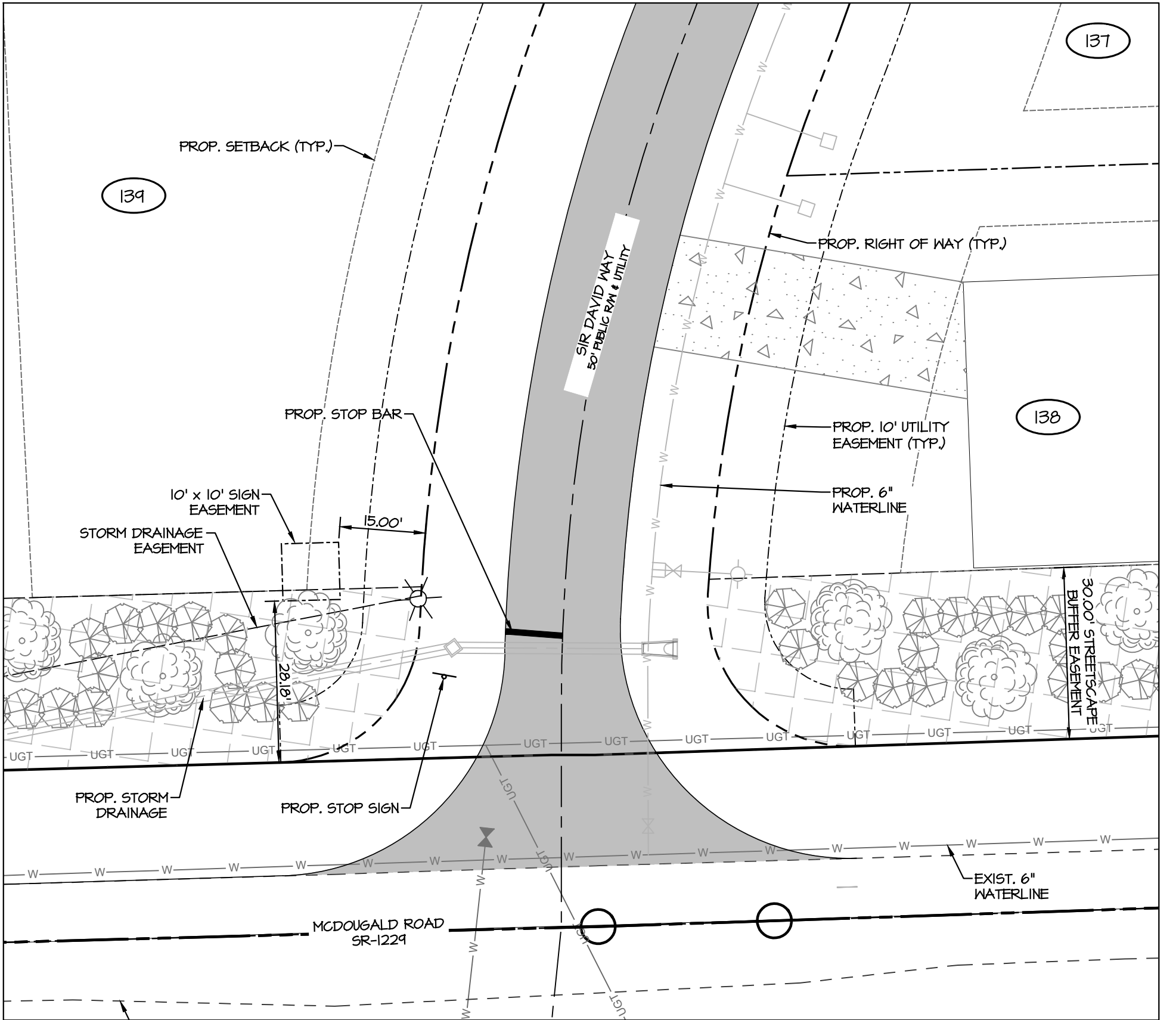
PLAN VIEW SCALE: 1" = 20'
