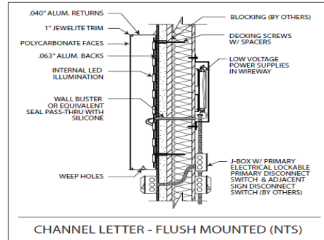
CHANNEL LETTER - FLUSH MOUNTED (NTS)
