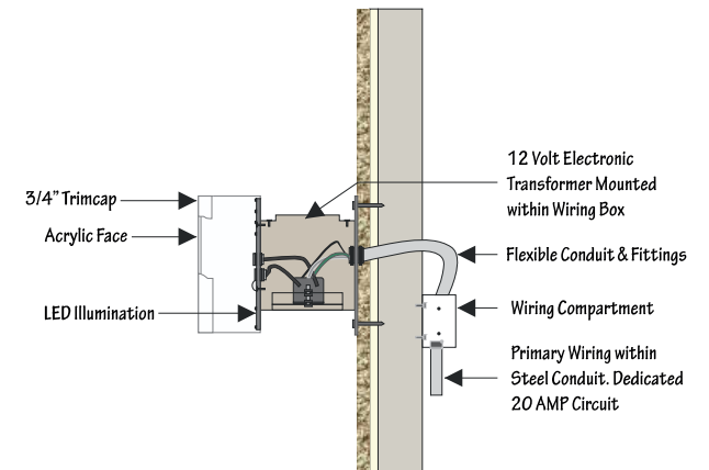
SIDE VIEW RACEWAY MOUNT
