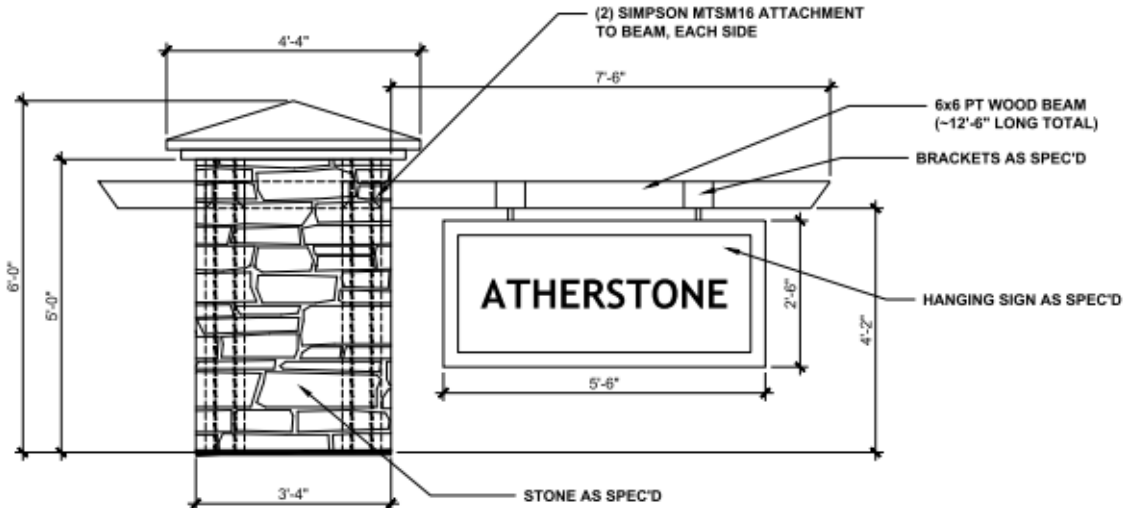
ELEVATION VIEW SCALE: 1/2" = 1'-0"
