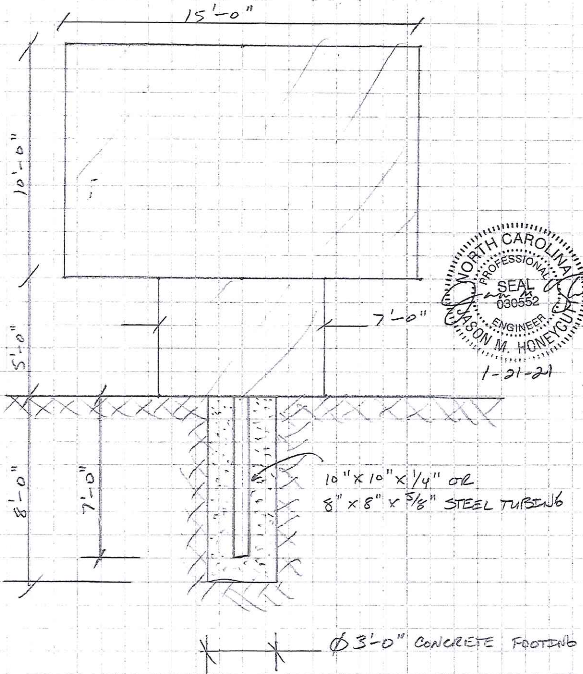
POLE + FOOTING DETAILS SCALE: 1/4" → 1'0" SIGN BY OTHERS
