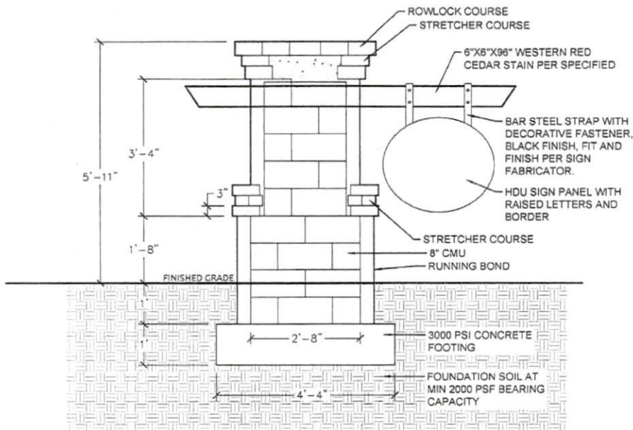
SECTION DETAIL
