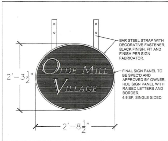
○ SIGN PANEL DETAIL SCALE: 1"=1'
