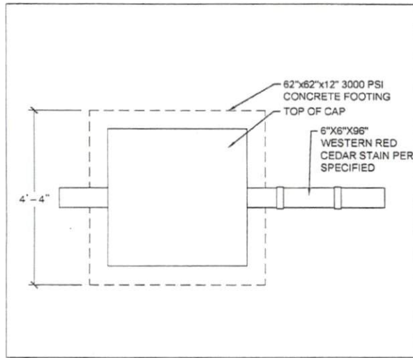
○ SIGN CROSS SECTION SCALE: \frac{1}{2} "=1'
