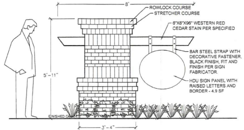
FRONT ELEVATION DETAIL
