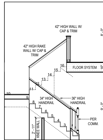
STAIR SECTION
