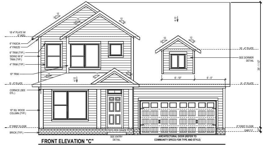
FRONT ELEVATION "C"
