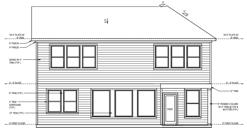
REAR ELEVATION "C"
