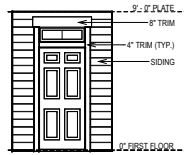
ENTRY DOOR DETAIL SCALE: 1/8" = 1'-0"
