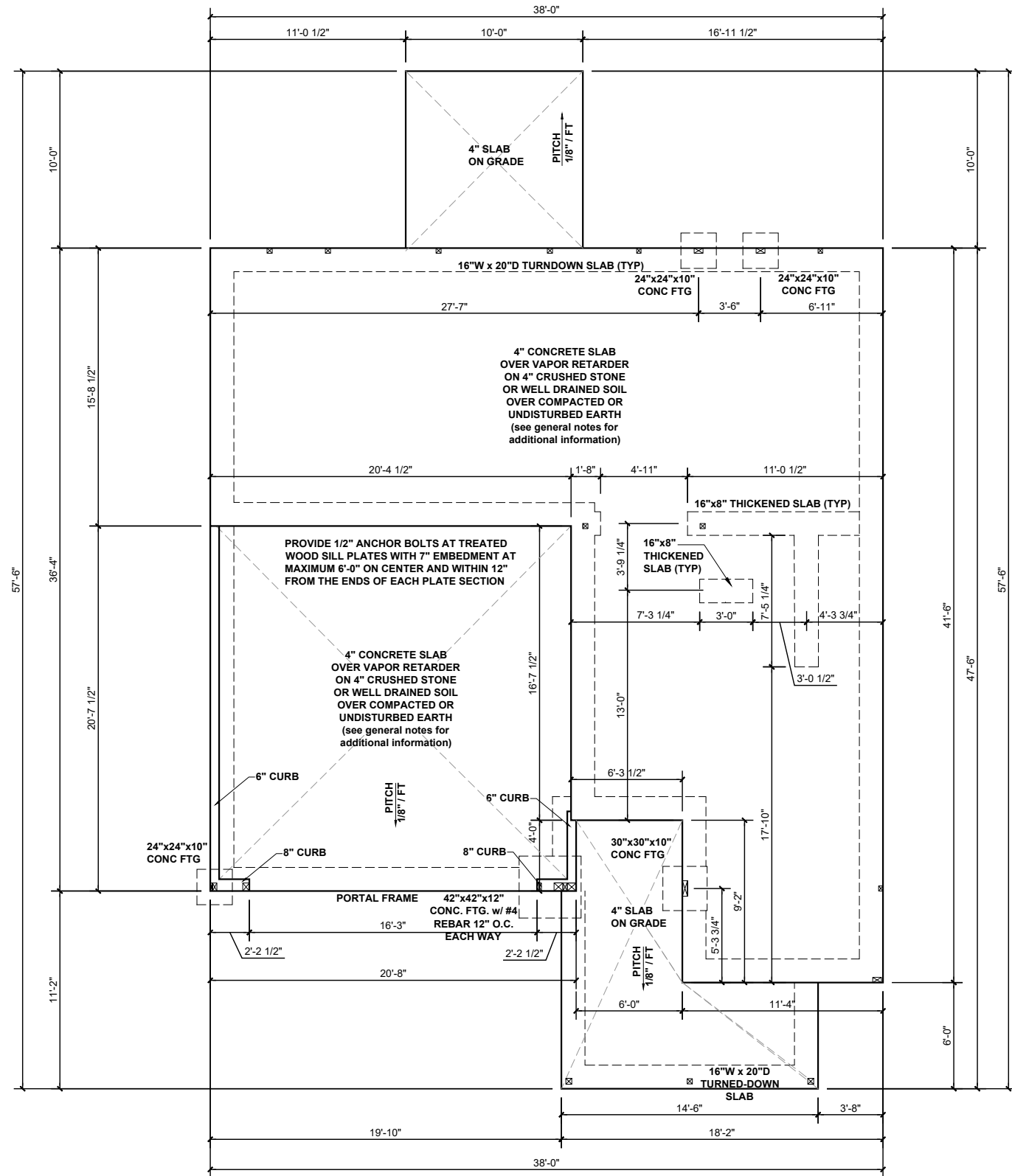
SLAB FOUNDATION PLAN - 'N' SCALE: 1/8"=1'-0"
