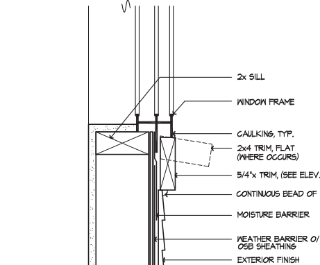
WINDOW SILL
