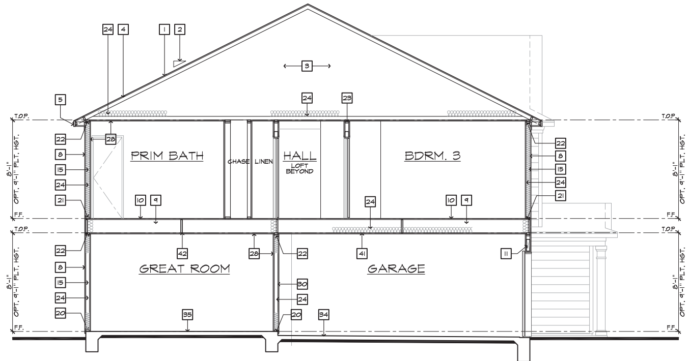
SECTION "B"
