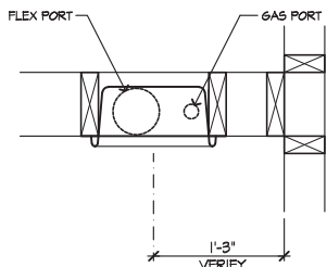
PLAN VIEW
