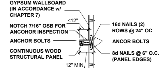
B) GARAGE T-WALL PORTAL FRAMING 16"-12"
