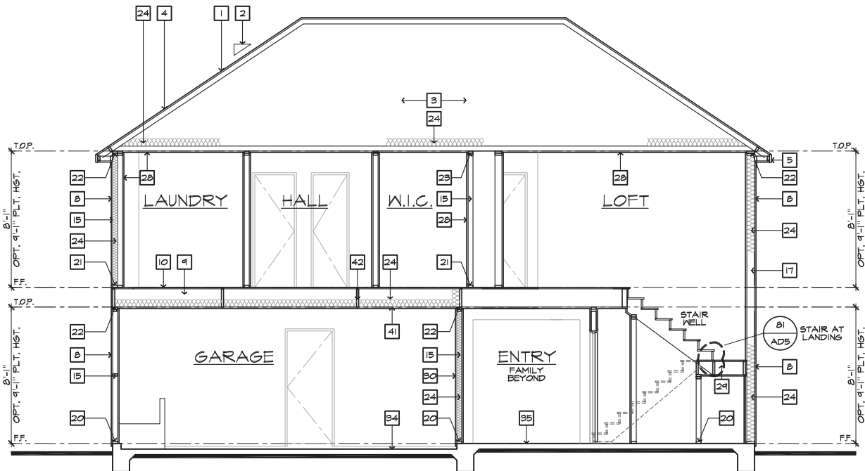
SECTION "C"
