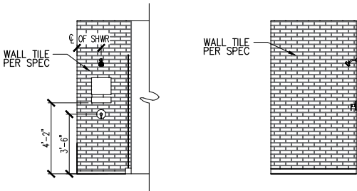
TYPICAL SHOWER NICHE AT SHOWER DETAIL 3/16"=1'-0"
