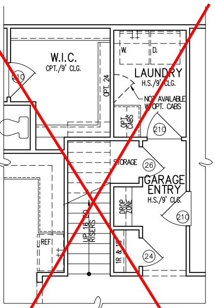
OPT. SECOND FLOOR STAIR PARTIAL FLOOR PLAN
