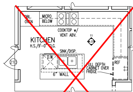
OPT. GOURMET 2 KITCHEN - PARTIAL PARTIAL FLOOR PLAN
