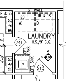
OPT. DOOR FROM PRIM. W.I.C TO LAUNDRY PARTIAL FLOOR PLAN
