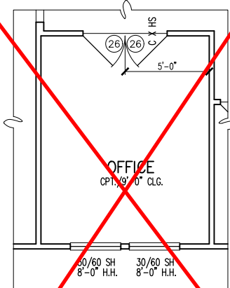
OPT. OFFICE ILO FLEX SPACE PARTIAL FLOOR PLAN
