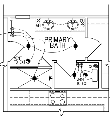
OPT. PRIMARY BATH 1 PARTIAL ELECTRICAL PLAN
