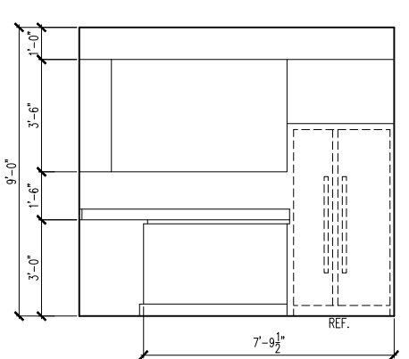
2 KITCHEN
