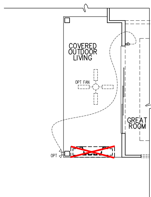
OPT. 12080 MULTI SLIDE DOOR AT GREAT ROOM PARTIAL ELECTRICAL PLAN 1/8"=1'-0"
