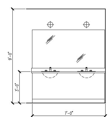
4 PRIMARY BATH
