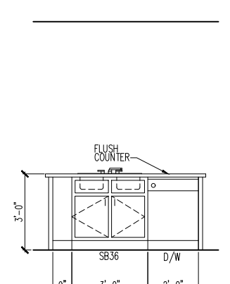
3 KITCHEN ISLAND
