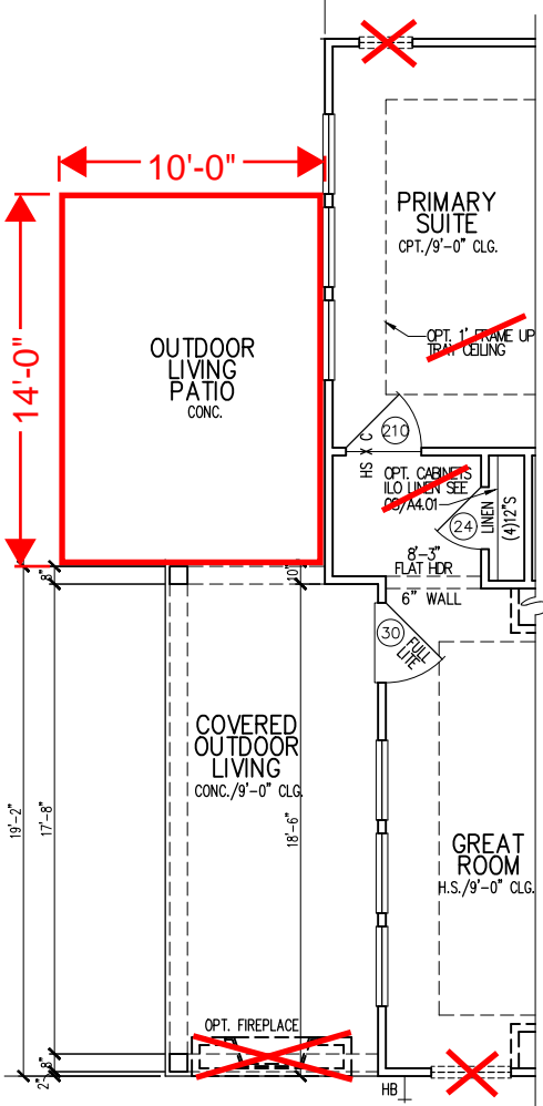
OPT. OUTDOOR LIVING PATIO PARTIAL FLOOR PLAN
