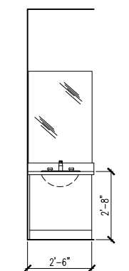
9 BATH 2
