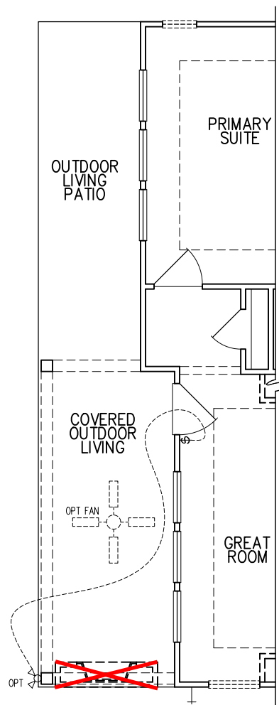
OPT. OUTDOOR LIVING PATIO PARTIAL ELECTRICAL PLAN 1/8"=1'-0"
