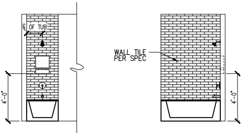
TYPICAL SHOWER NICHE AT TUB SHOWER DETAIL 3/16"=1'-0"
