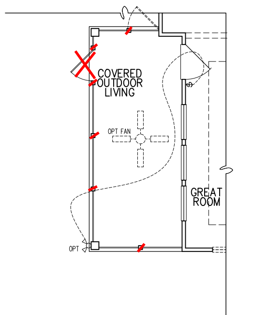
OPT. SCREENED COVERED OUTDOOR LIVING PARTIAL ELECTRICAL PLAN 1/8"=1'-0"
