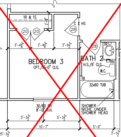
OPT. BEDROOM 3 ILO FLEX SPACE PARTIAL FLOOR PLAN
