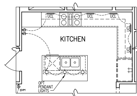
OPT. GOURMET 1 KITCHEN - PARTIAL ELECTRICAL PLAN 1/8"=1'-0"
