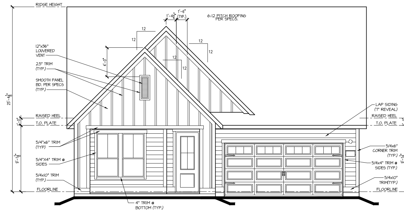
FRONT ELEV. "A" 1/8"=1'-0"
