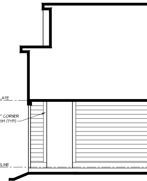
RIGHT INSIDE PORCH ELEV. "A" 1/8"=1'-0"
