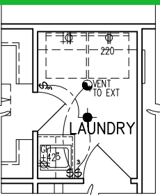
OPT. DOOR FROM PRIM. W.I.C TO LAUNDRY PARTIAL ELECT. PLAN
