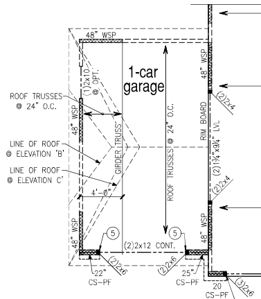
PARTIAL FRAMING PLAN OPTIONAL 1-CAR CARRIAGE GARAGE
