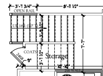
Optional Open Rail ILO 45° Wall w/ Cap
