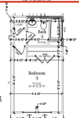
Optional Bed 5 & Bath 3 ILO Study
