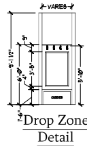
Optional Drop Zone at Garage Entry
