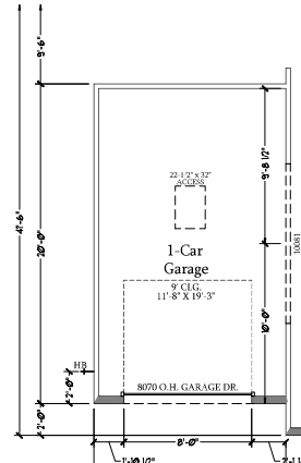
Optional 1-Car Carriage Garage
