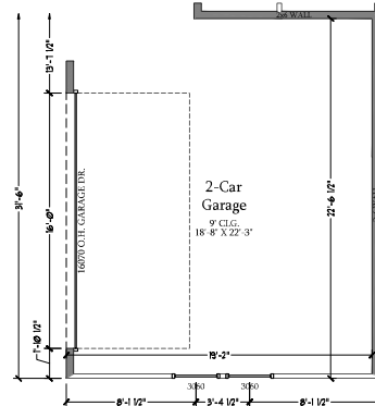
Optional 2-Car Side Load Garage
