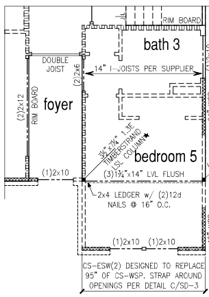
PARTIAL FRAMING PLAN OPTIONAL BED 5 & BATH 3 I/O STUDY
