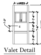
Valet Detail
