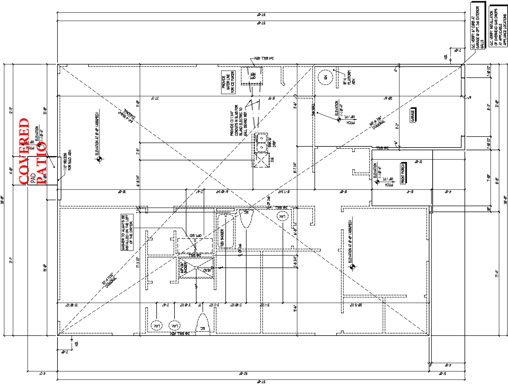
SCALE 1/4" = 1'-0"
