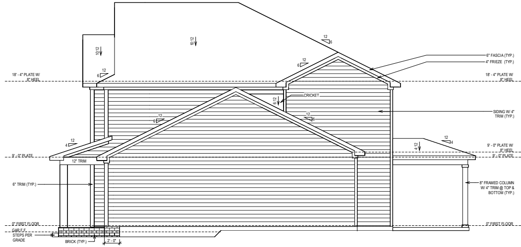
SIDE ELEVATION "A"
