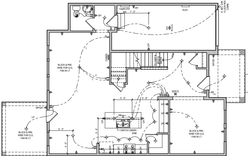
FIRST FLOOR "A"
