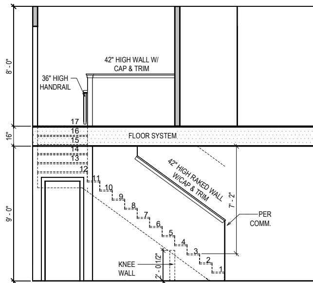
STAIR SECTION
