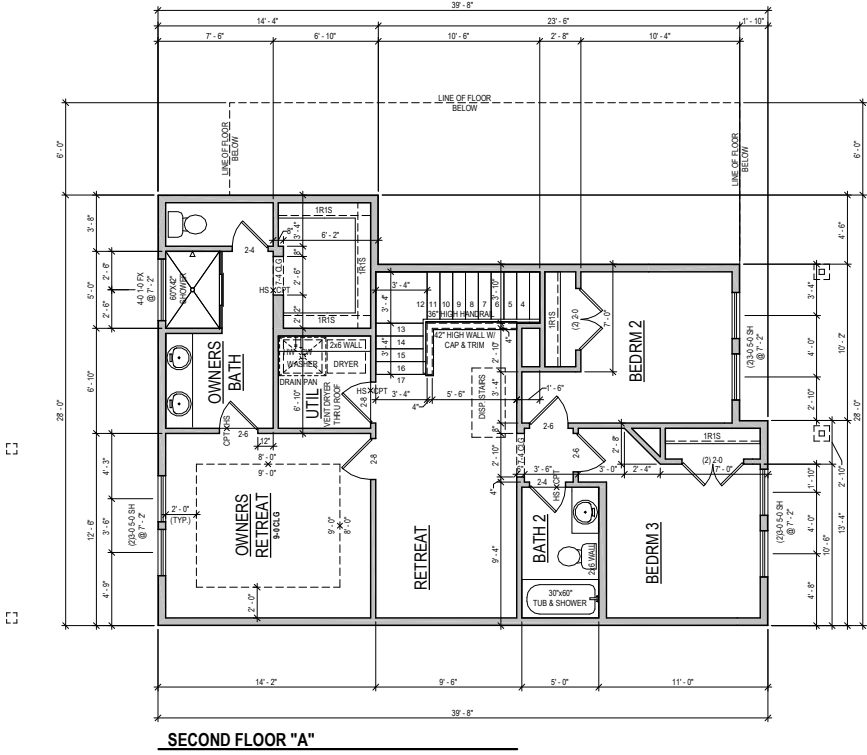
SECOND FLOOR "A"
