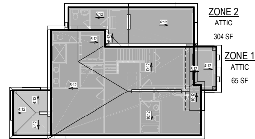
VENTILATION PLAN "A"
