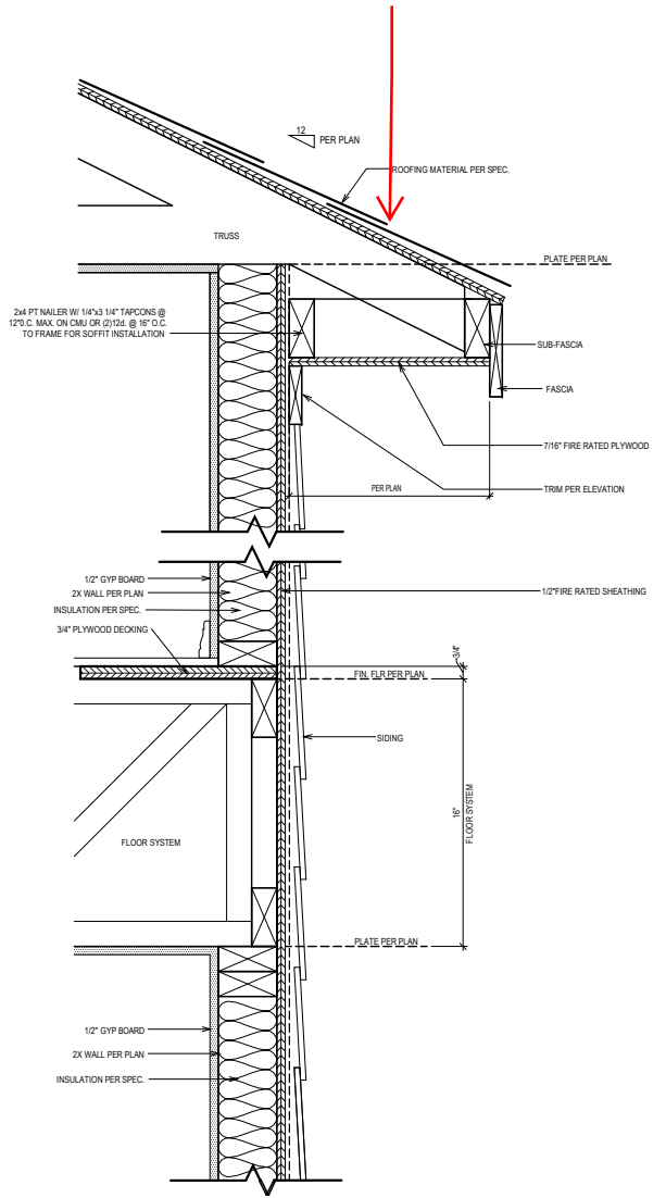
WALL SYSTEM @ FRAME WALL - SIDING
