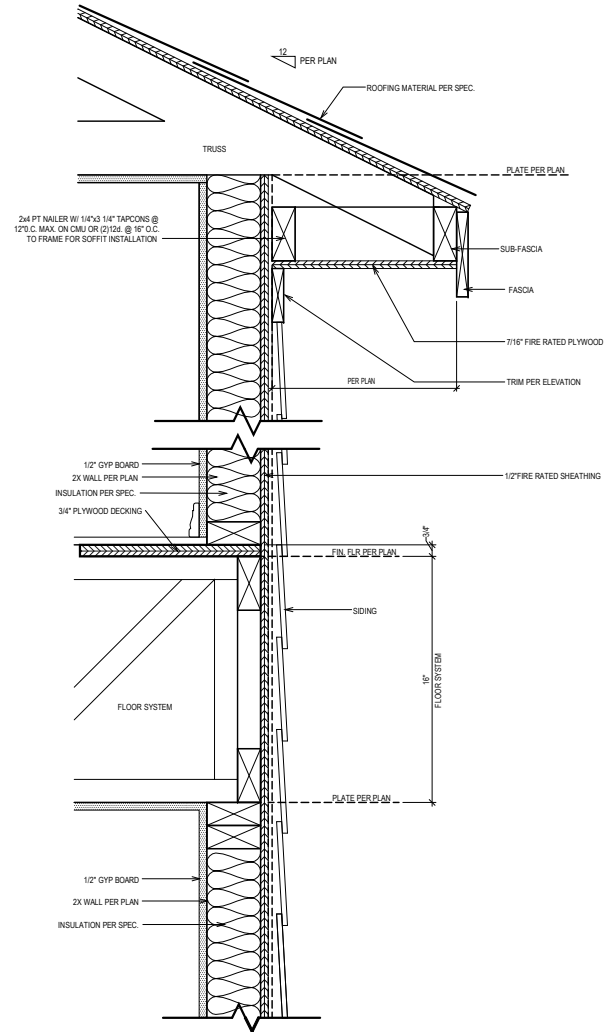
WALL SYSTEM @ FRAME WALL - SIDING
