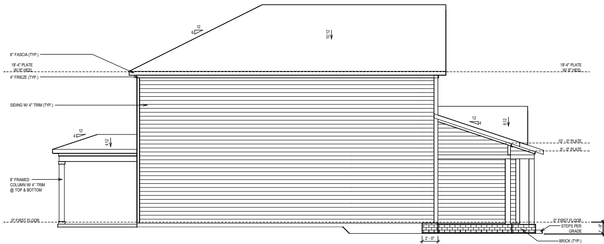
SIDE ELEVATION "B"
