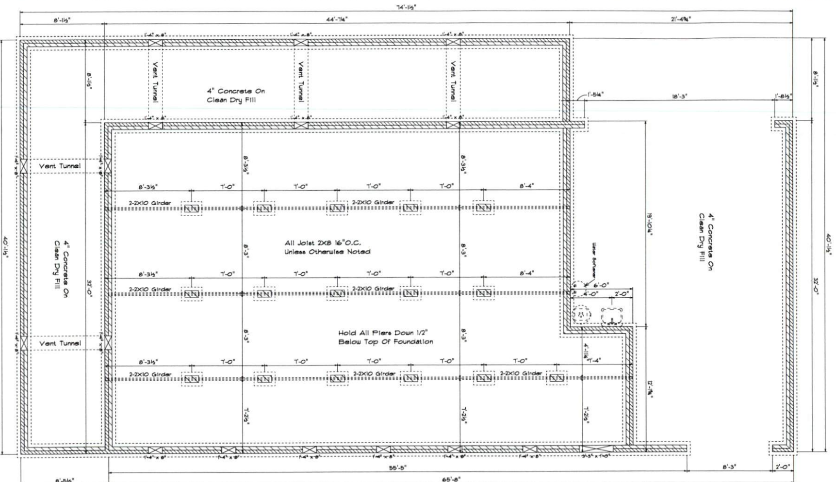
Foundation Plan
