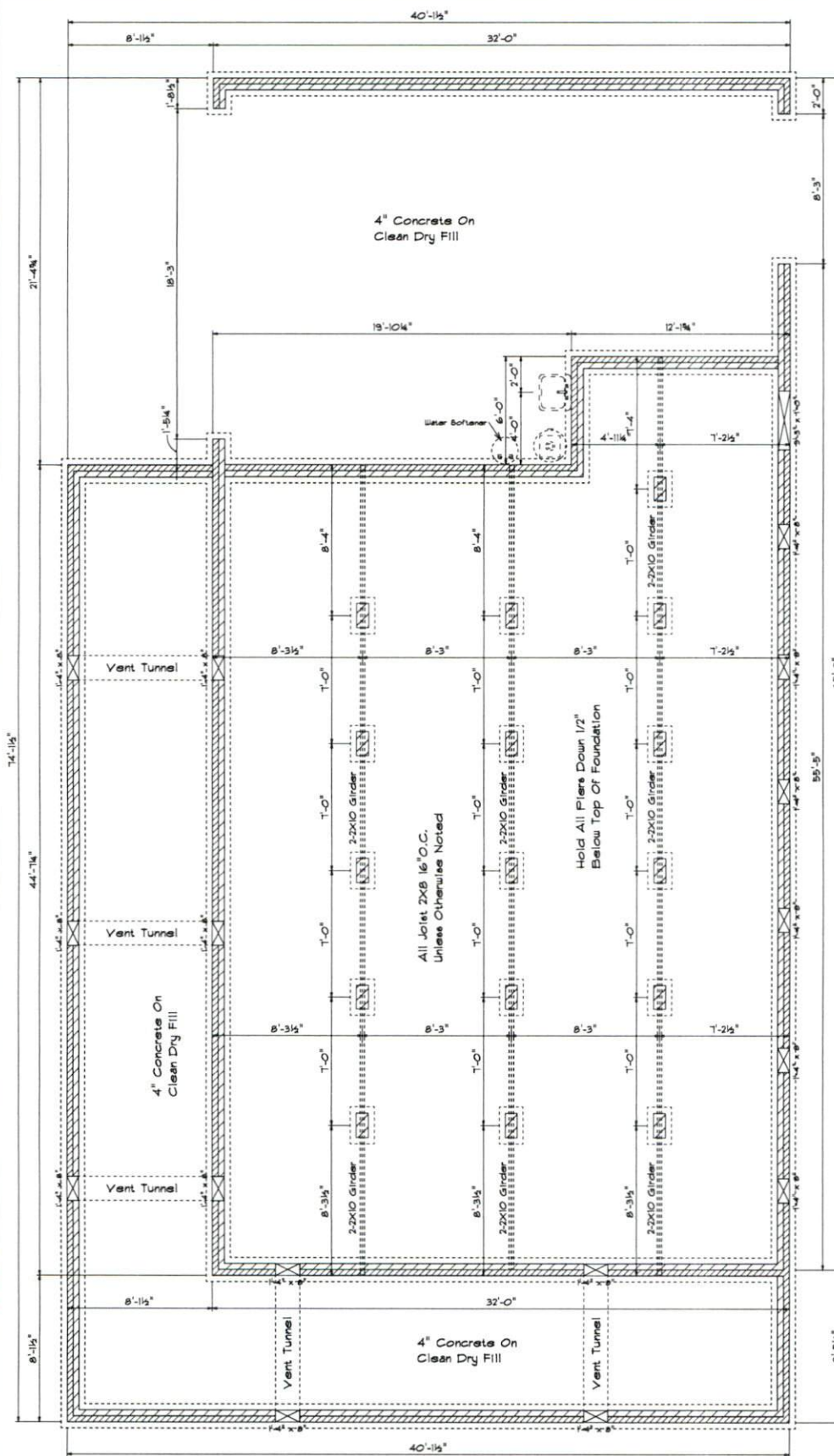
Foundation Plan
