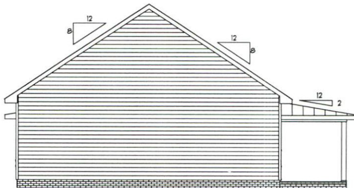
Rear Elevation Scale: 3/16" = 1'0"
