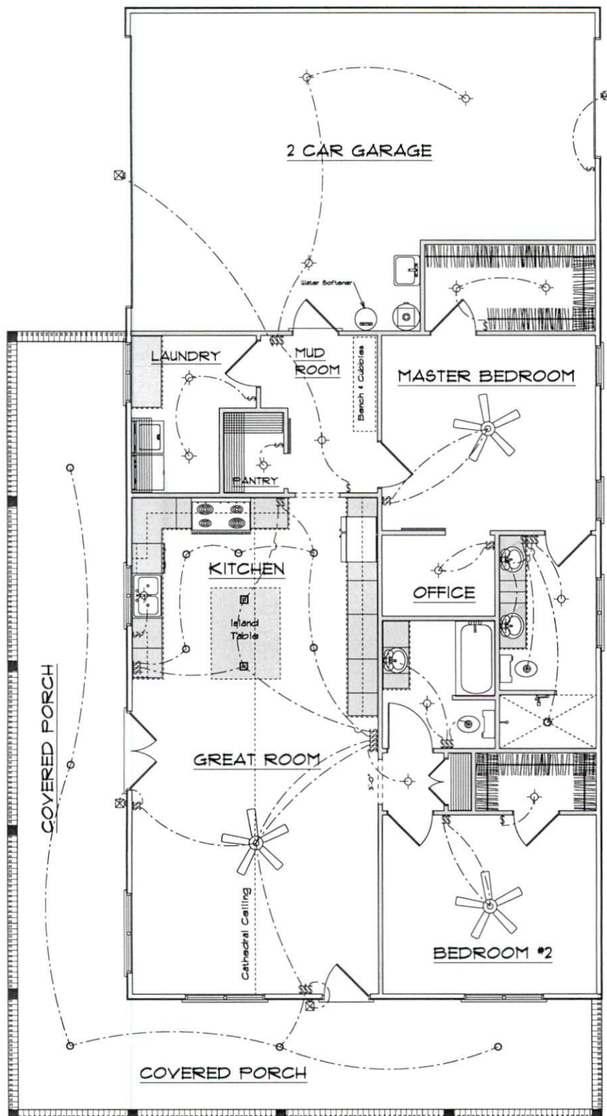
Electrical Plan
