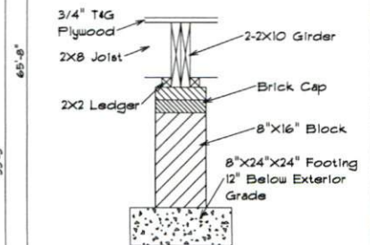
Footing & Pier Detail
