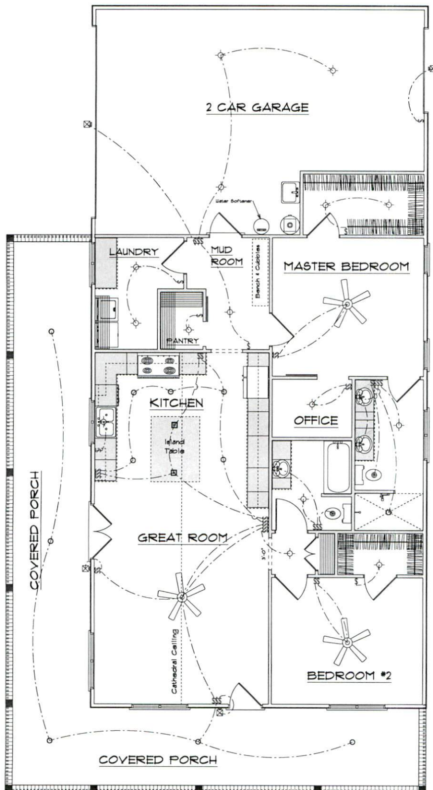
Electrical Plan
