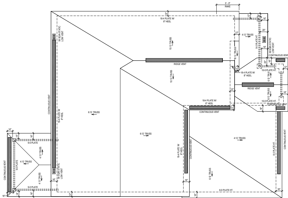
ROOF PLAN
