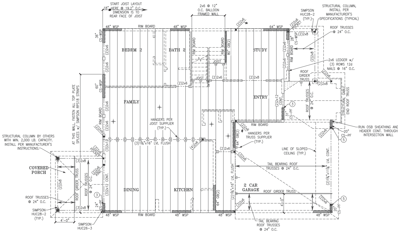
SECOND FLOOR FRAMING PLAN
