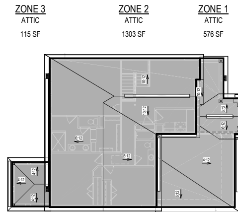
VENTILATION PLAN
