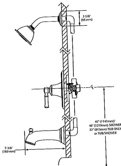
THICK WALL APPLICATION
