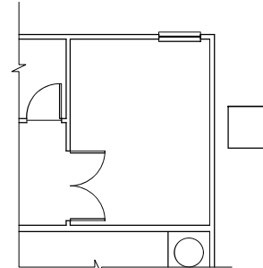
OPT BI-SWING DOORS AT STUDY SCALE 1/4" = 1'-0"
