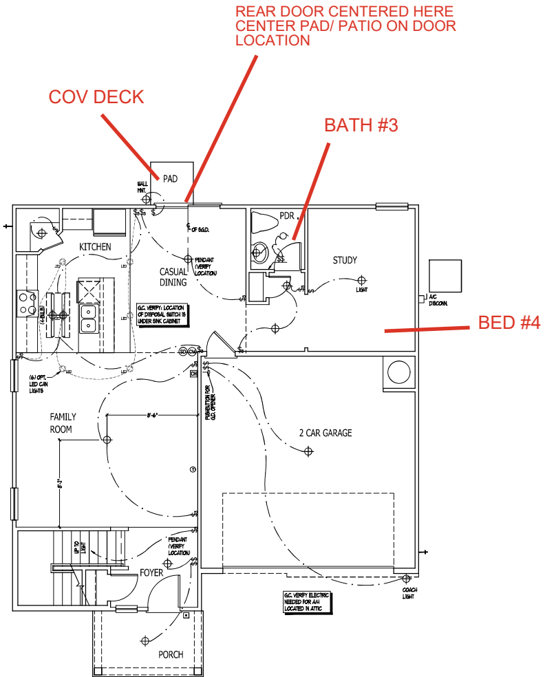
FIRST FLOOR PLAN-A
