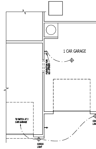
OPT 1 CAR GARAGE SCALE 1/4" = 1'-0"
