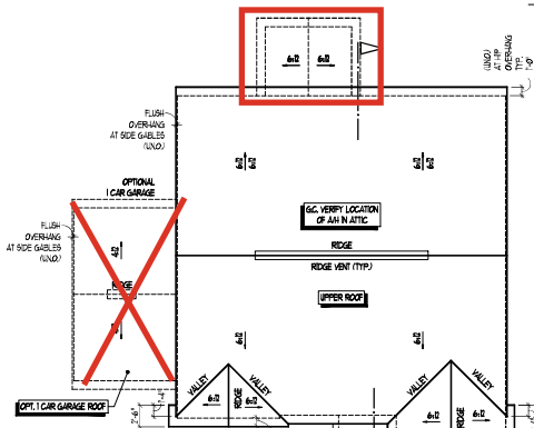
ROOF PLAN SCALE 1/8" = 1'-0"
