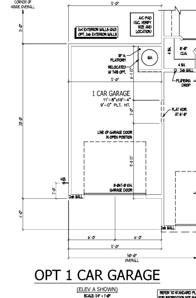
FIRST FLOOR PLAN OPTIONS
