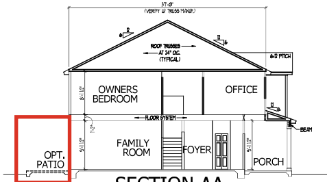
SECTION AA SCALE 1/8" = 1'-0"
