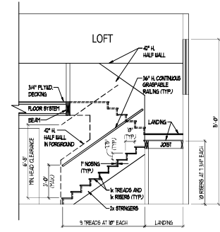
STAIR SECTION
