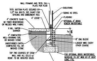
TYPICAL STEM WALL DETAIL (w/ OPTIONAL WATERBARRIER)
