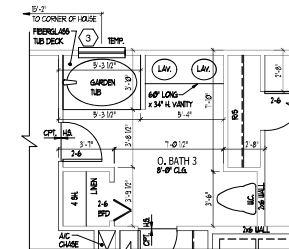
OPT OWNER'S BATH 3
