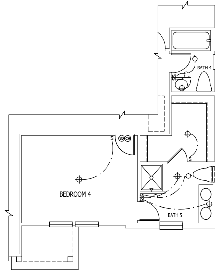
OPT BEDROOM 4/ BATH 5 ILO BEROOM 3 AND OFFICE SCALE 1/4" = 1'-0"
