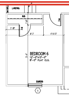
OPT BEDROOM 6 ILO LOFT
