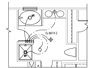
OPT OWNER'S BATH 2 SCALE 1/4" = 1'-0"
