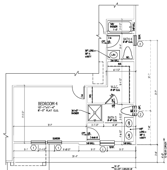
OPT BEDROOM 4/ BATH 5 ILO BEROOM 3 AND OFFICE
