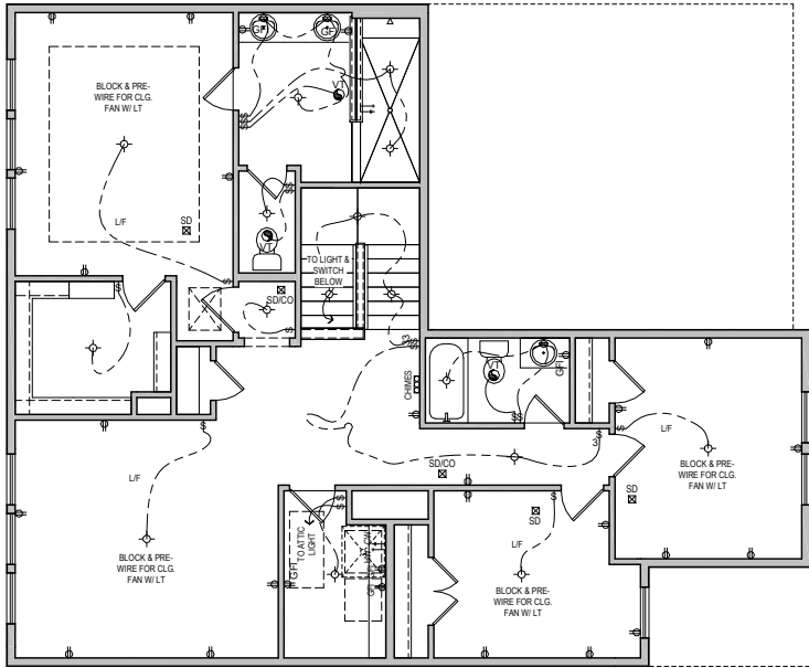
SECOND FLOOR "B"
