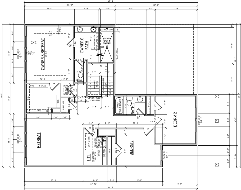
SECOND FLOOR "B"
