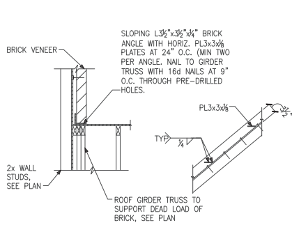
A PENT ROOF DETAIL CURVED ROOF
