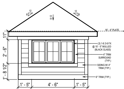
DORMER DETAIL "B" SCALE: 1/4" = 1'-0"
