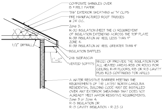
INSULATION DETAIL
