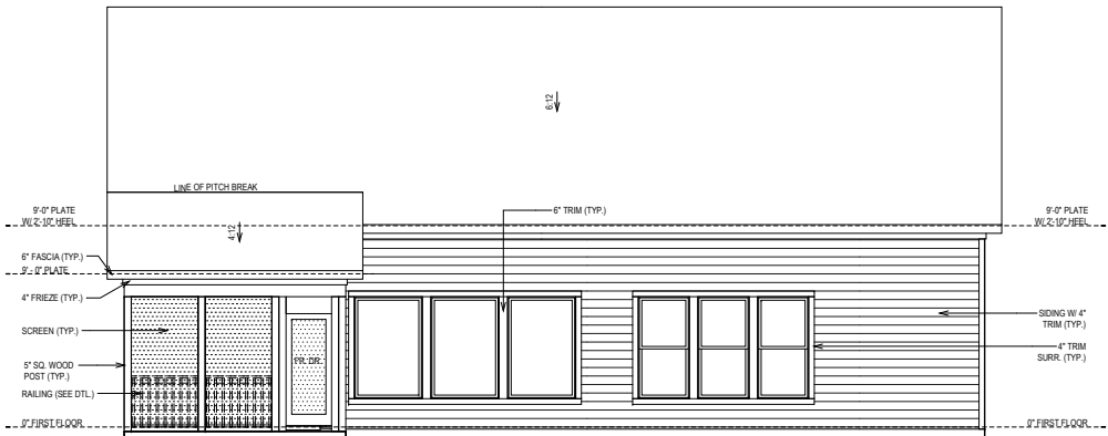
REAR ELEVATION "C"
