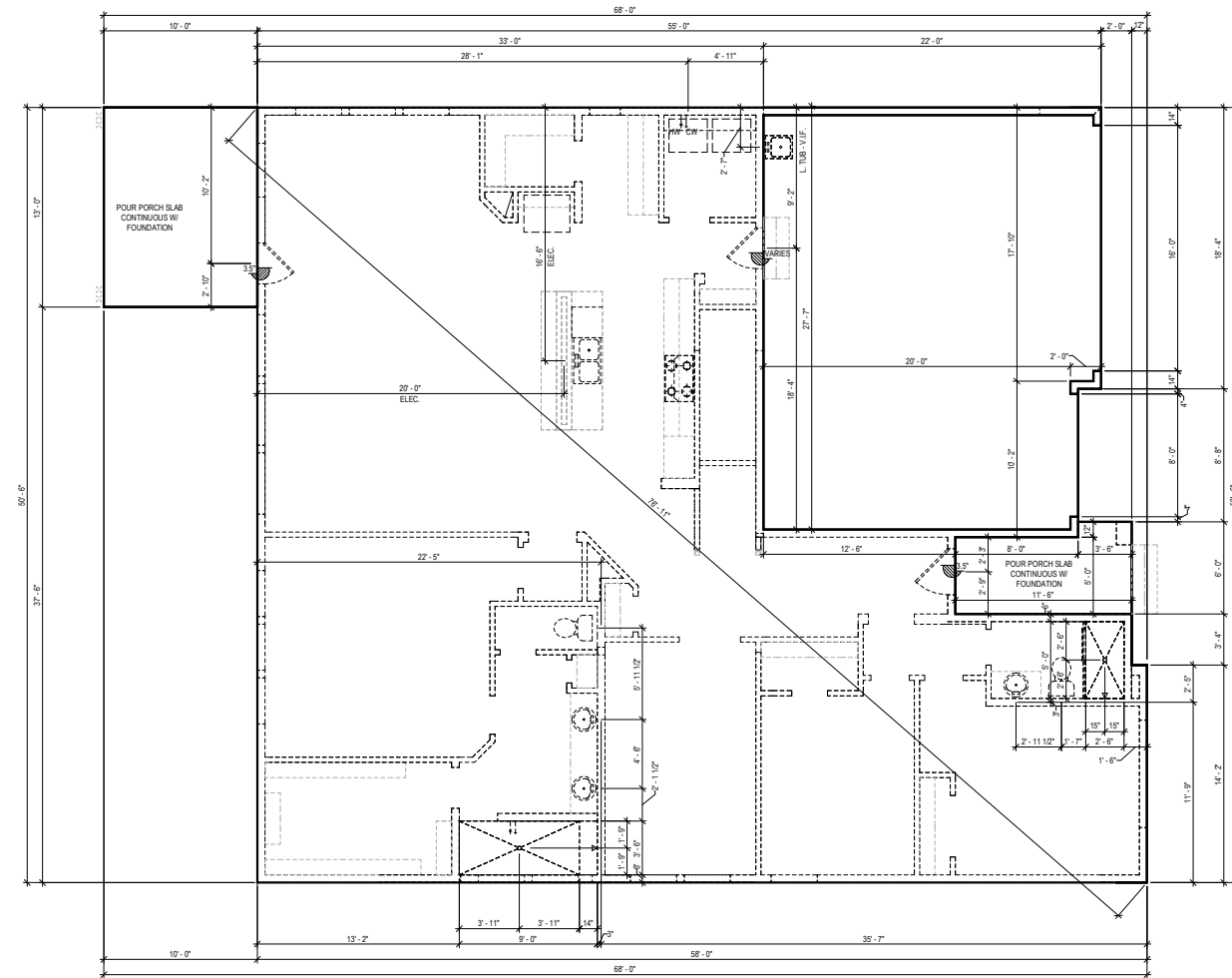
FIRST FLOOR "C"
