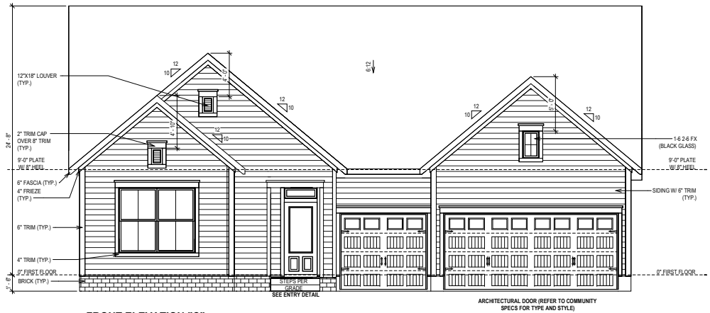
FRONT ELEVATION "C"
