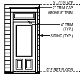
ENTRY DETAIL
