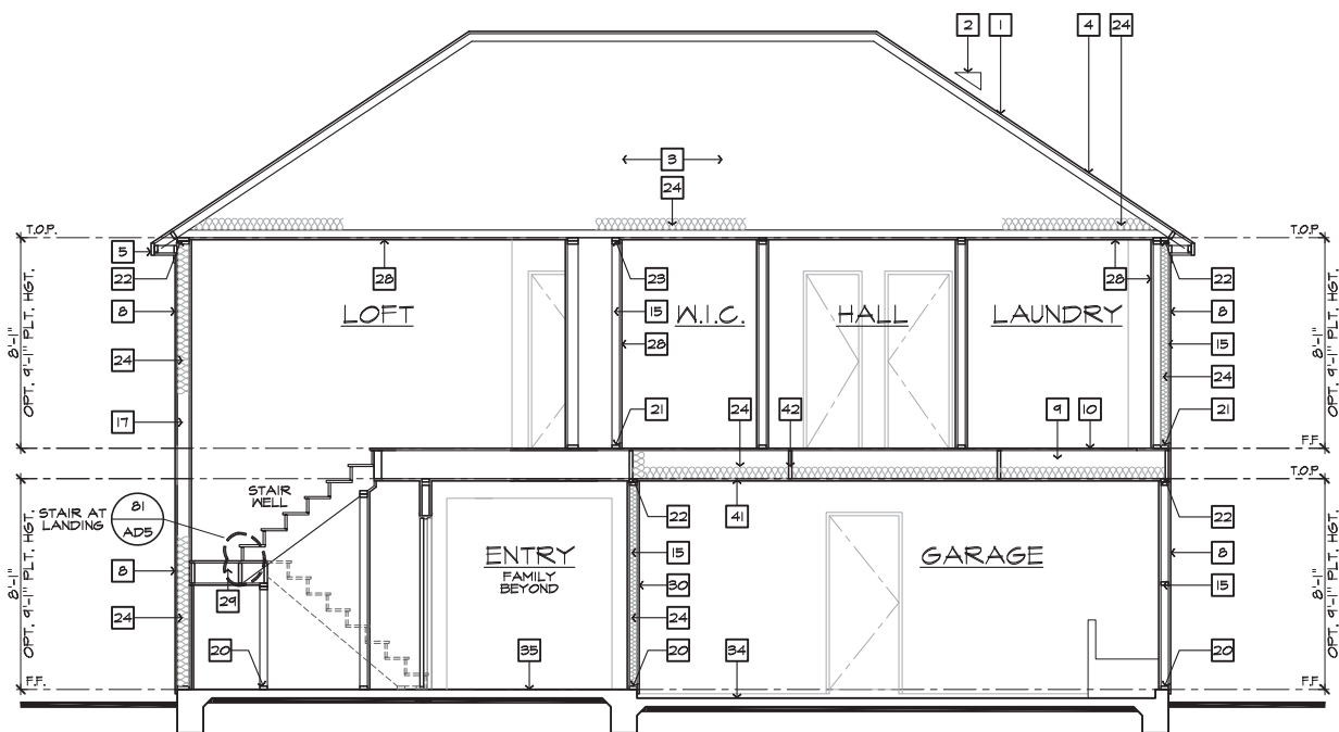
SECTION "C"
