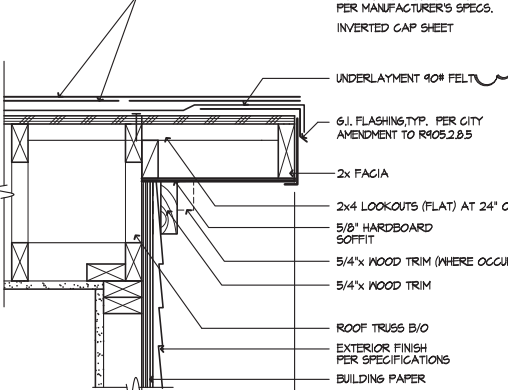
RAKE SCALE 1 1/2"=1'-0" 0732-04q
