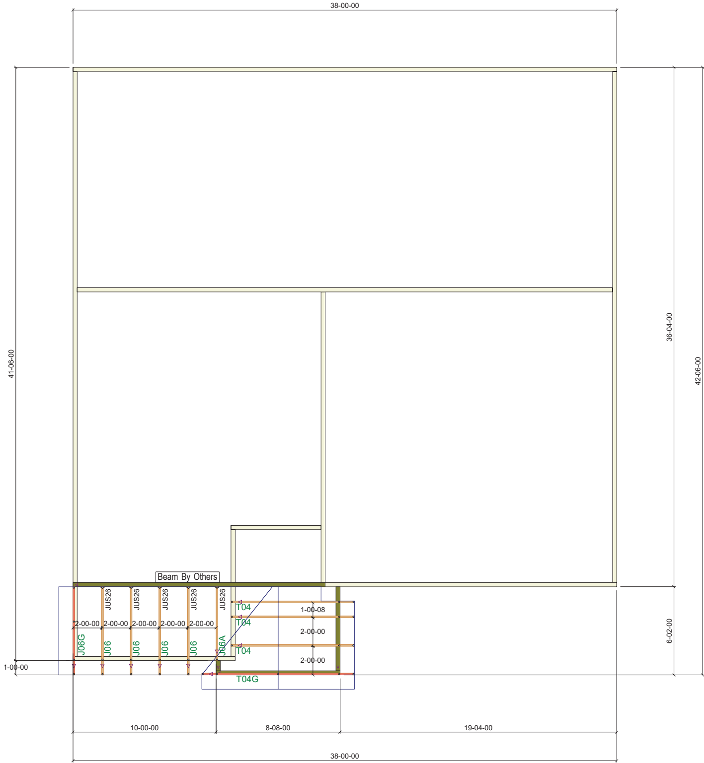
FLOOR PLAN M
