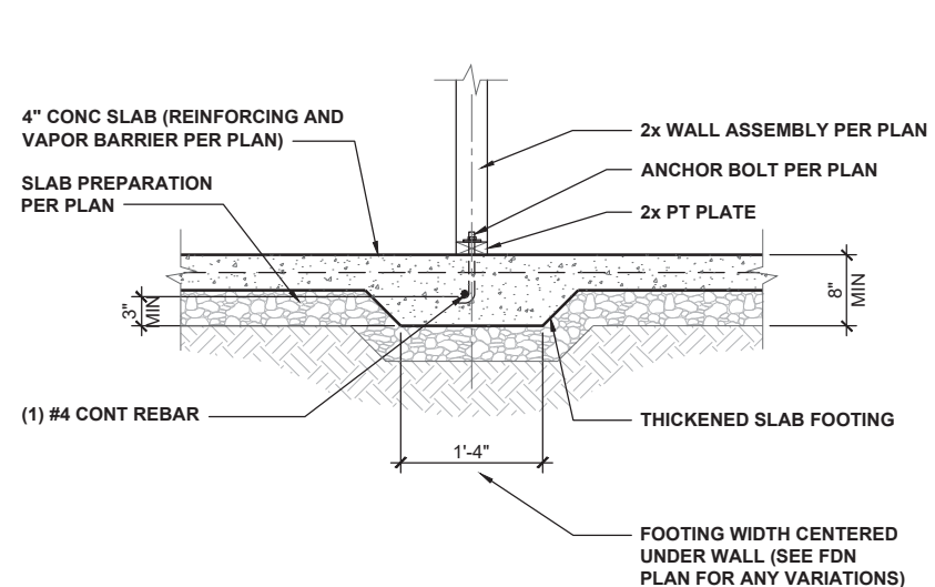
INTERIOR FOOTING 1/2" = 1'-0" 7
