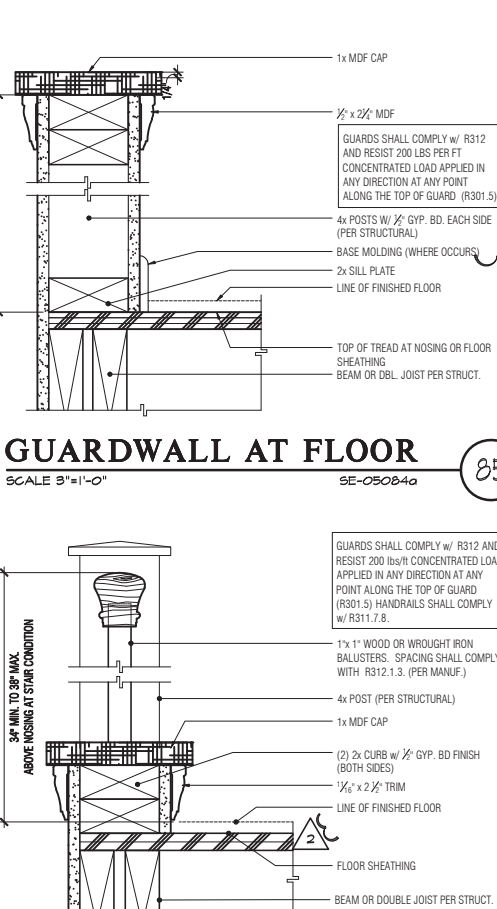
GUARDRAIL
