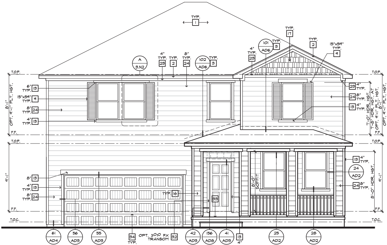
FRONT ELEVATION 'N' W/ CRAWL SPACE AT OPTIONAL 9'-1" PLT. HGT.
