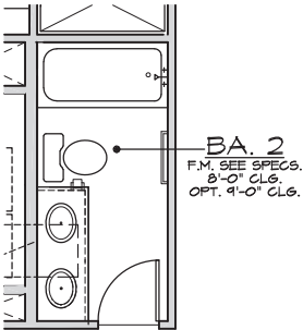
Dual Sinks AT BATH 2
