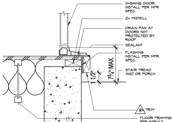
SWING DOOR THRESHOLD SCALE 3/8"=1'-0" AT CRAWL SPACE
