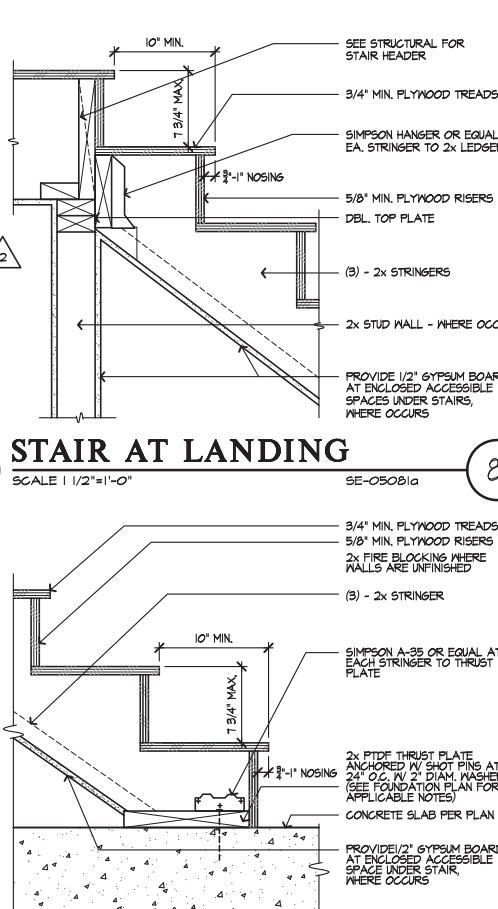
STAIR AT CONC. FLOOR
