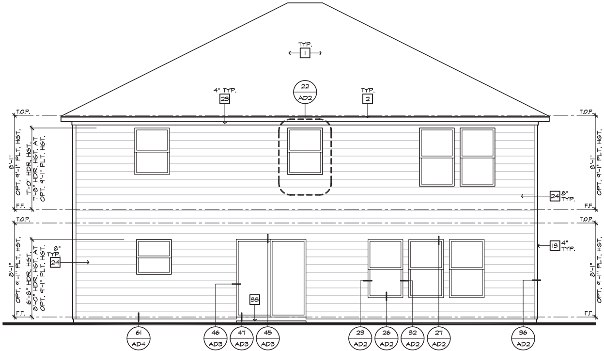
REAR ELEVATION 'N'
