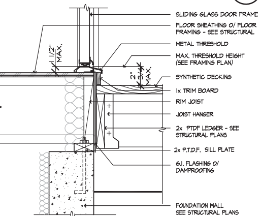
WALL @ DECK SCALE 3/8"=1'-0"
