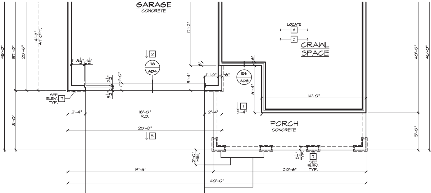
PARTIAL CRAWL SPACE PLAN 'N'
