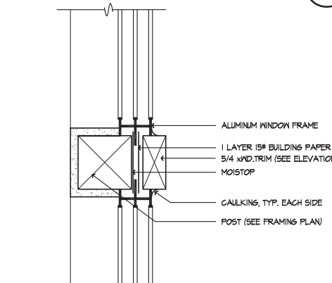
VERT. WINDOW MULL.
