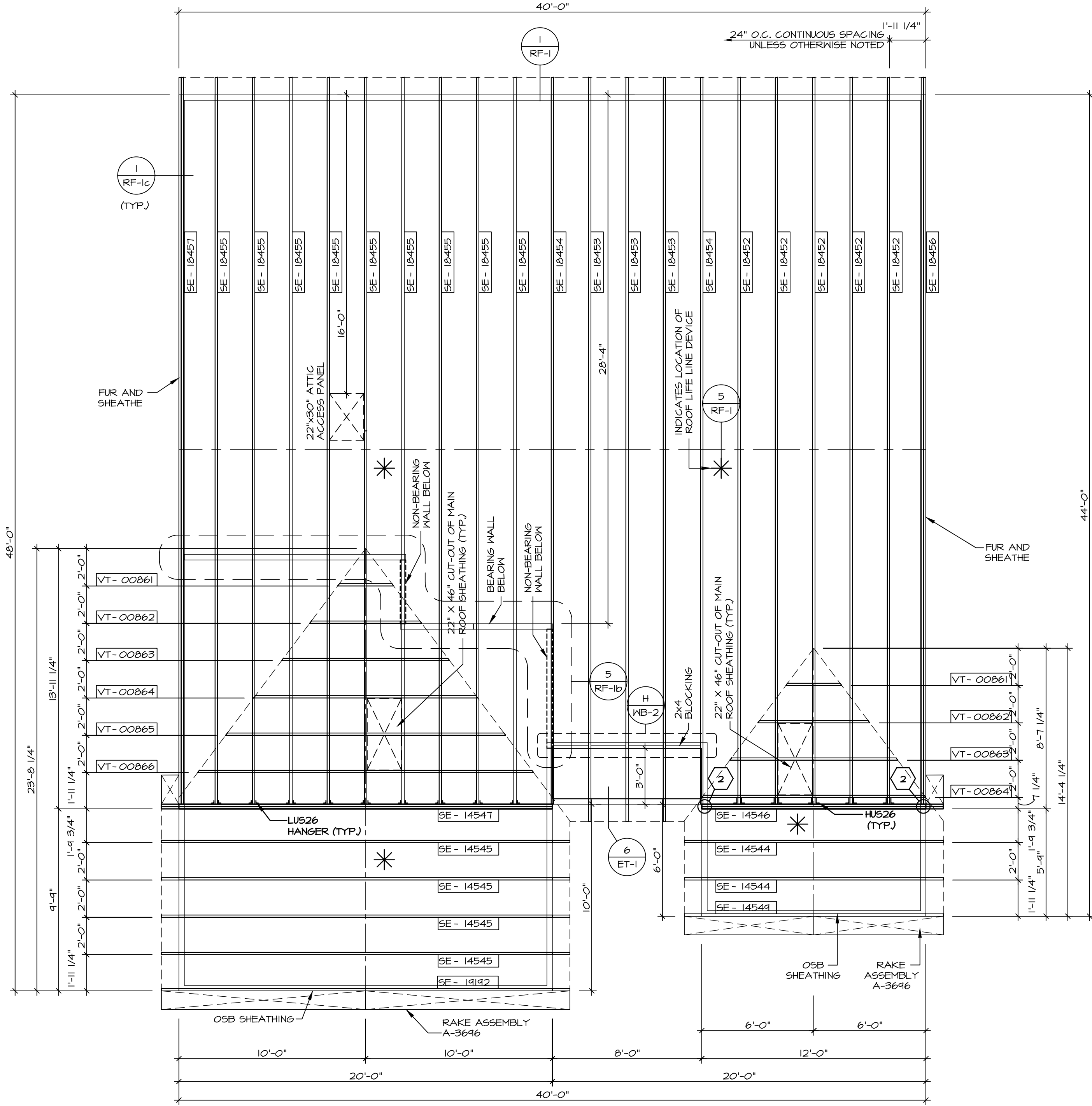
ROOF FRAMING SCALE: 1/4" = 1'-0"
