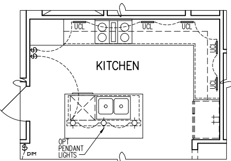
OPT. GOURMET 1 KITCHEN - PARTIAL ELECTRICAL PLAN
