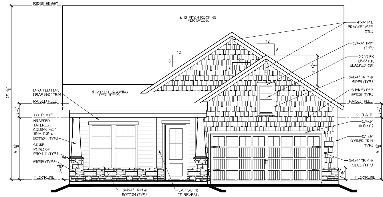
FRONT ELEV. "C" 1/8"=1'-0"
