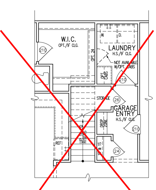
OPT. SECOND FLOOR STAIR PARTIAL FLOOR PLAN
