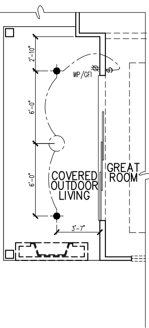
OPT. 12080 MULTI SLIDE DOOR AT GREAT ROOM PARTIAL ELECTRICAL PLAN
