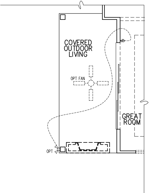
OPT. 12080 MULTI SLIDE DOOR AT GREAT ROOM PARTIAL ELECTRICAL PLAN
