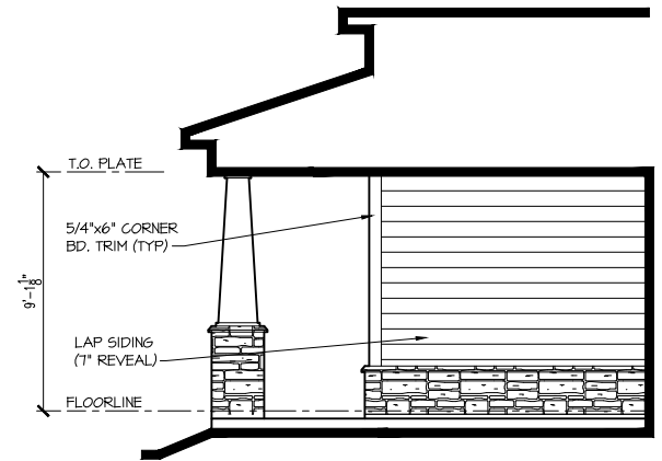
RIGHT INSIDE PORCH ELEV. "C" 1/8"=1'-0"
