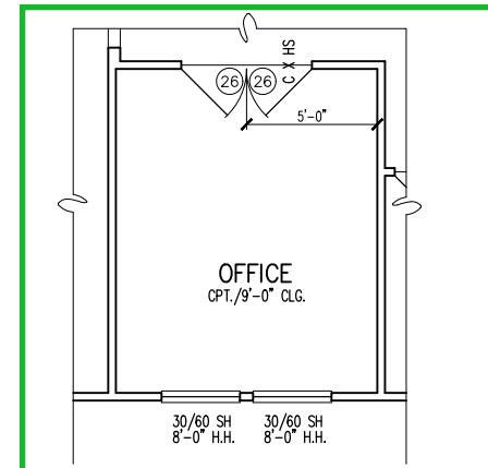
OPT. OFFICE ILO FLEX SPACE PARTIAL FLOOR PLAN
