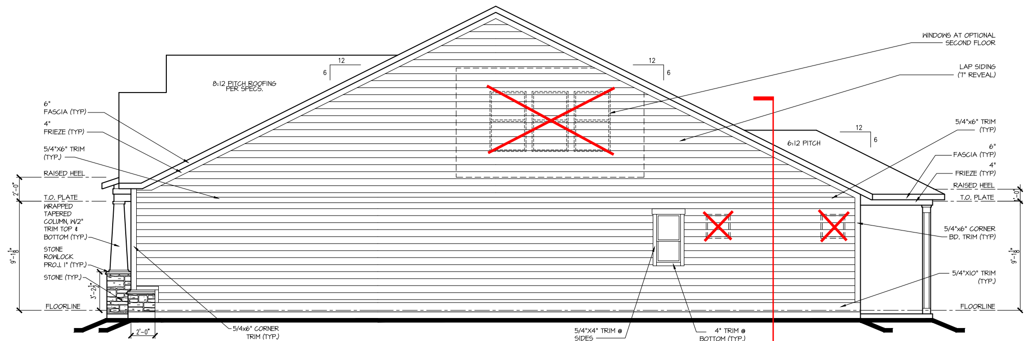
RIGHT ELEV. "C" 1/8"=1'-0"
