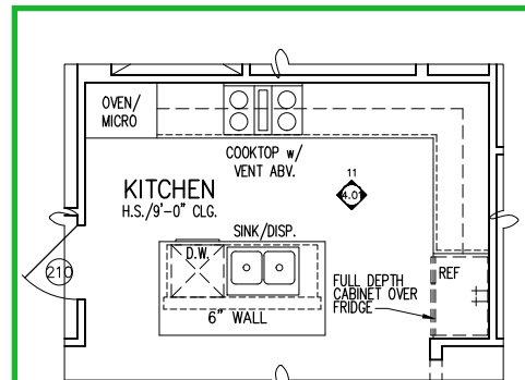
OPT. GOURMET 1 KITCHEN - PARTIAL PARTIAL FLOOR PLAN
