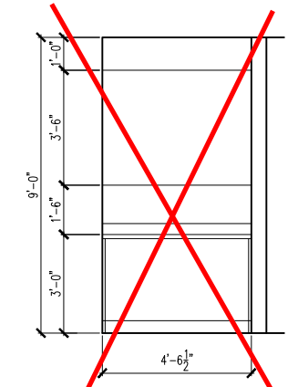
13 PRIMARY SUITE HALL 2 w/ OPT CABINETS
