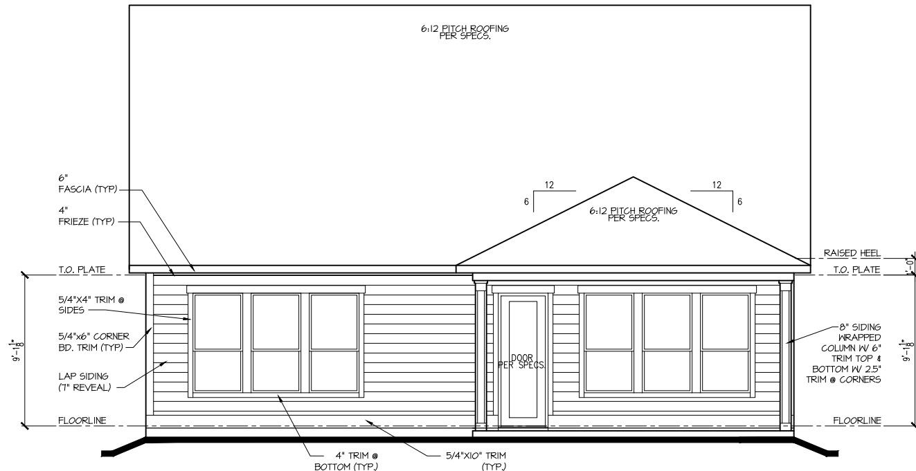
REAR ELEV. "C" 1/8"=1'-0"
