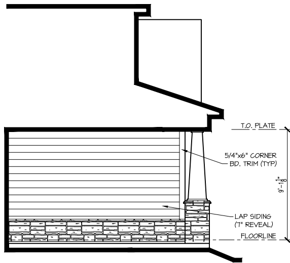
LEFT INSIDE PORCH ELEV. "C" 1/8"=1'-0"
