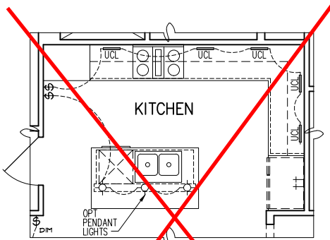
OPT. GOURMET 2 KITCHEN - PARTIAL ELECTRICAL PLAN
