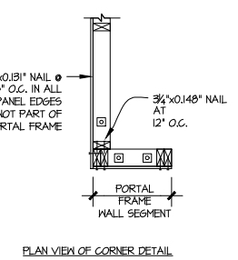
PLAN VIEW OF CORNER DETAIL
