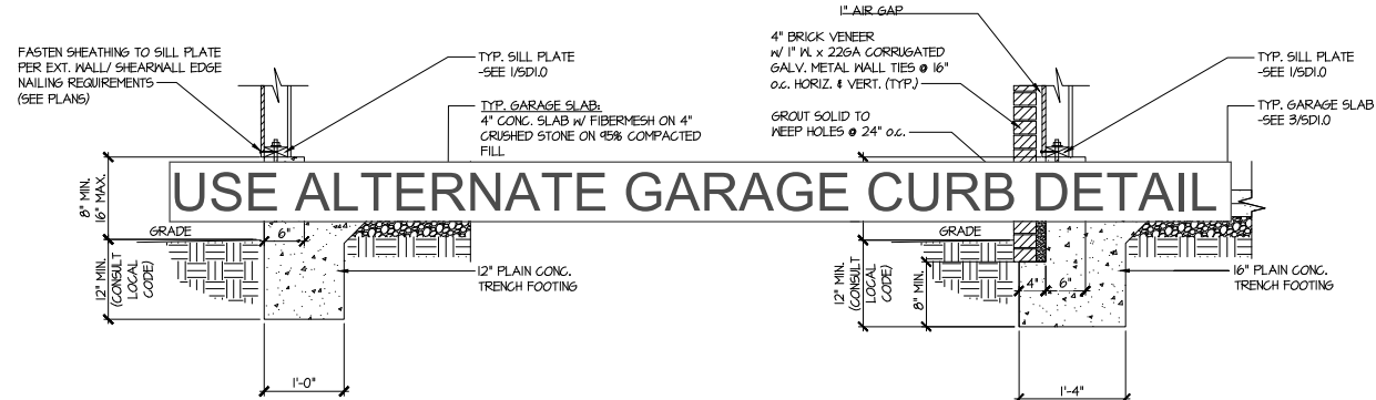
3 TYPICAL SLAB ON GRADE GARAGE PERIMETER FOOTING w/ BRICK VENEER
