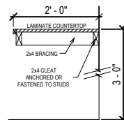
COUNTERTOP DETAIL SCALE: 1/2" = 1'-0"
