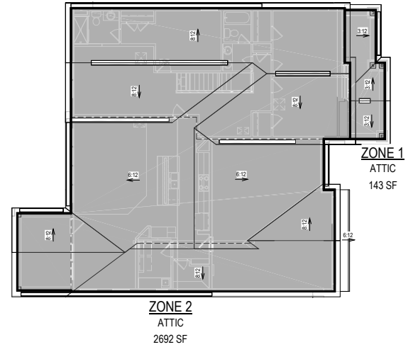
ATTIC VENTILATION "B"
