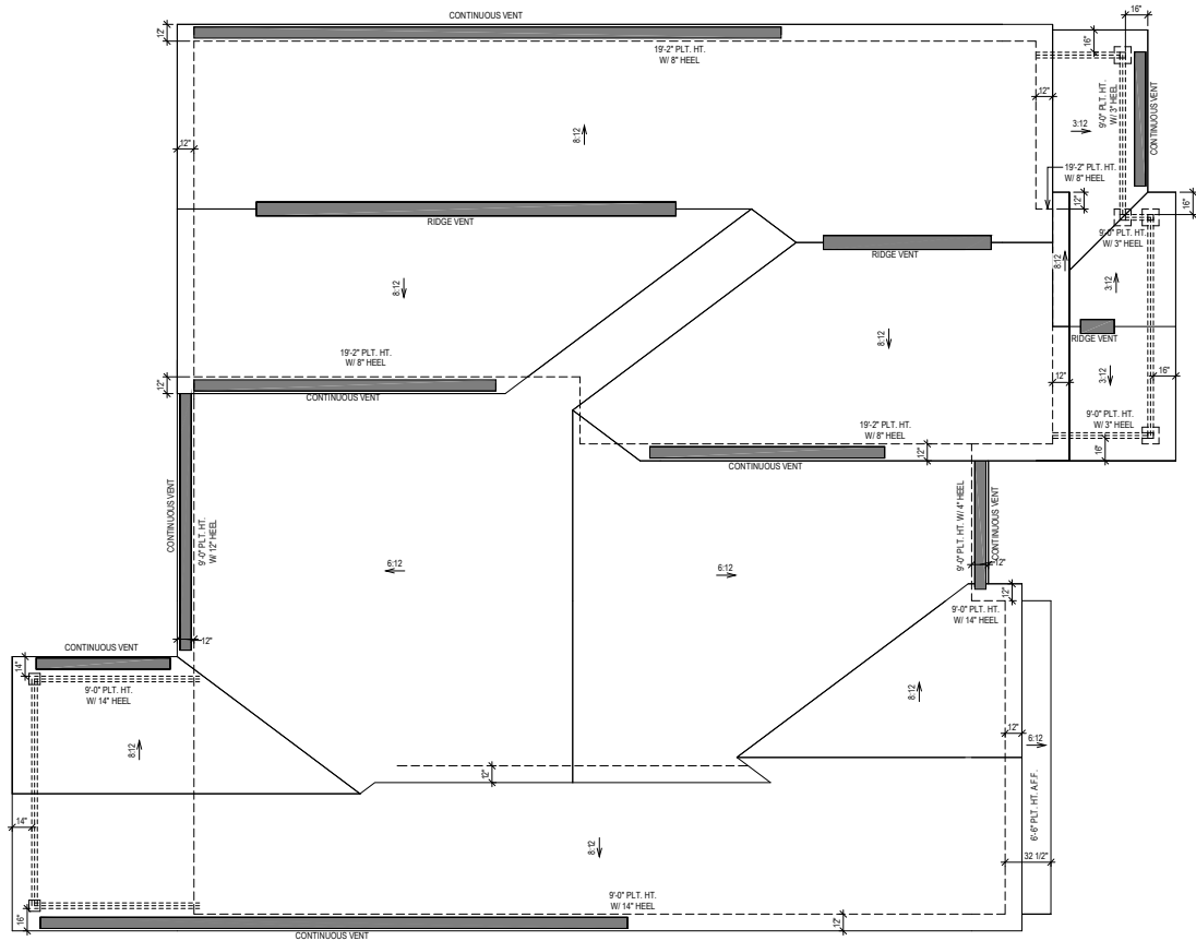
ROOF PLAN "B"
