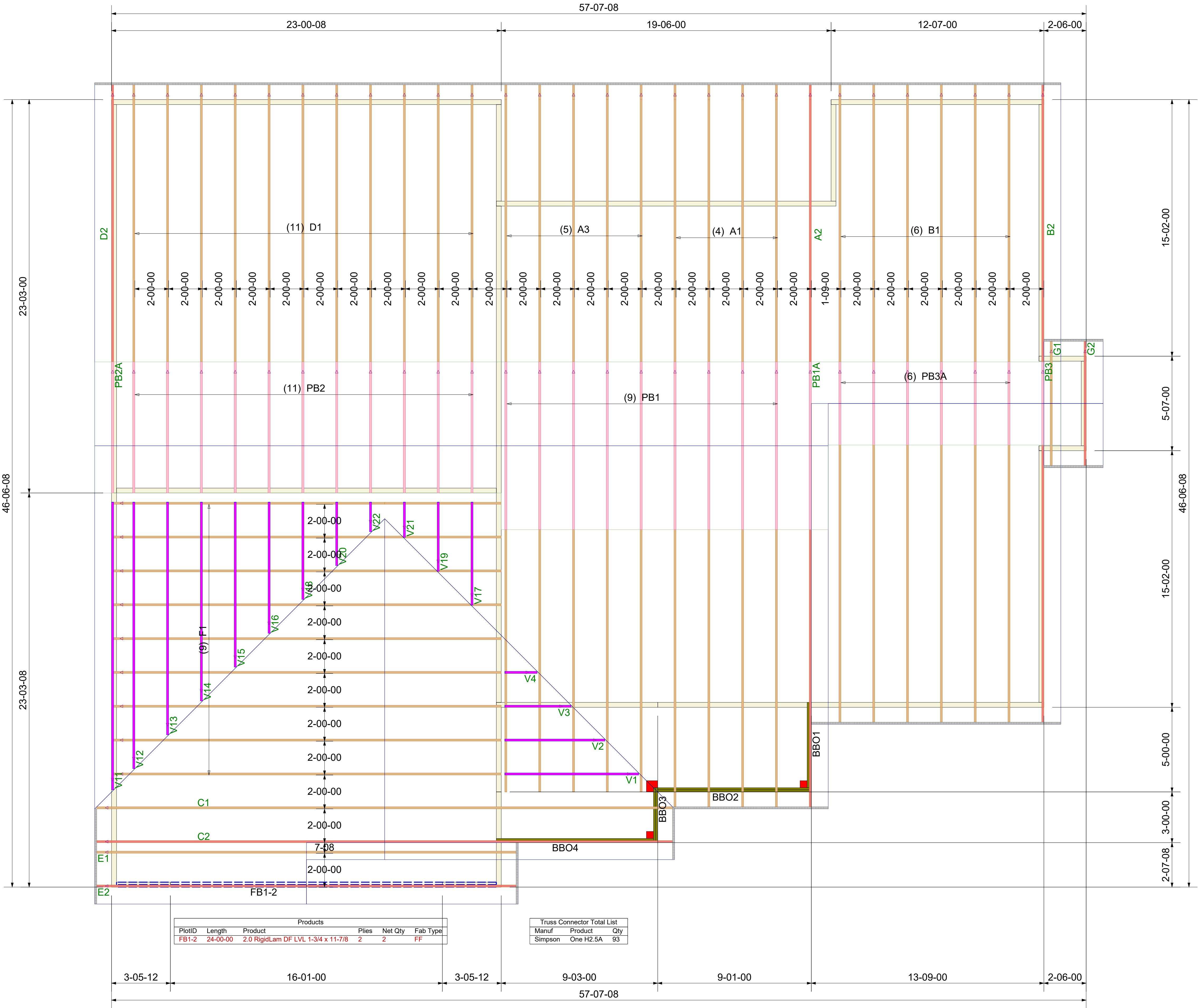
ROOF TRUSS FRAMING DRAWING SCALE : NTS
