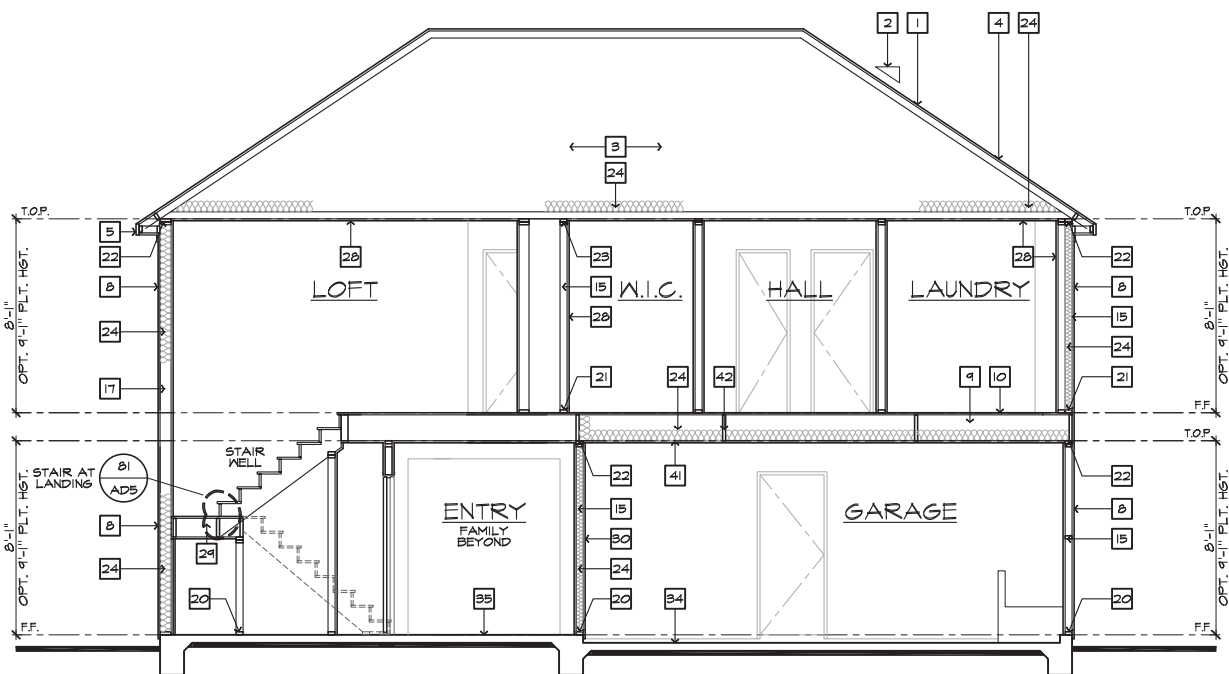
SECTION "C"
