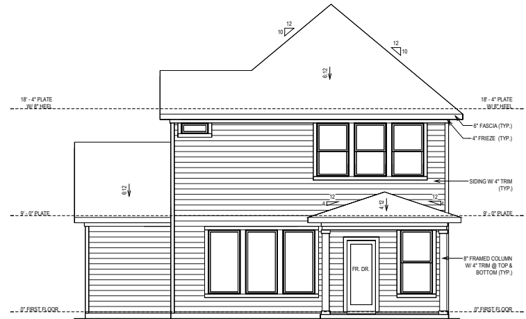
REAR ELEVATION "A"
