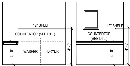
UTILITY
