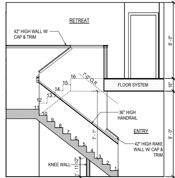
STAIR SECTION
