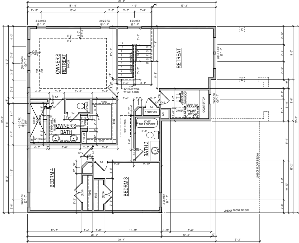
SECOND FLOOR "B"
