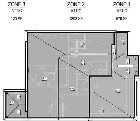
VENTILATION PLAN "B"
