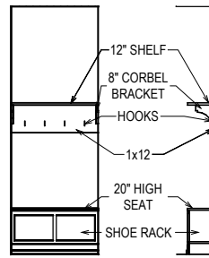
BACKPACK RACK
