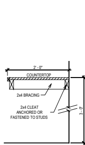
COUNTERTOP DETAIL SCALE: 1/2" = 1'-0"
