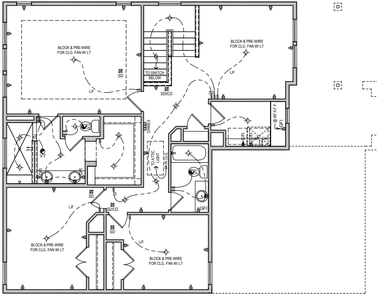
SECOND FLOOR "B"
