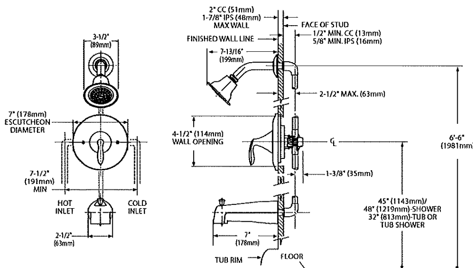
THICK WALL APPLICATION
