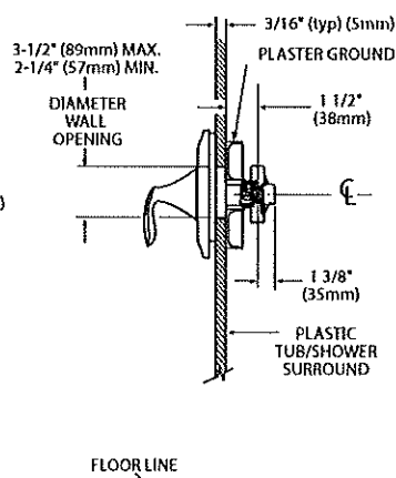
THIN WALL APPLICATION
