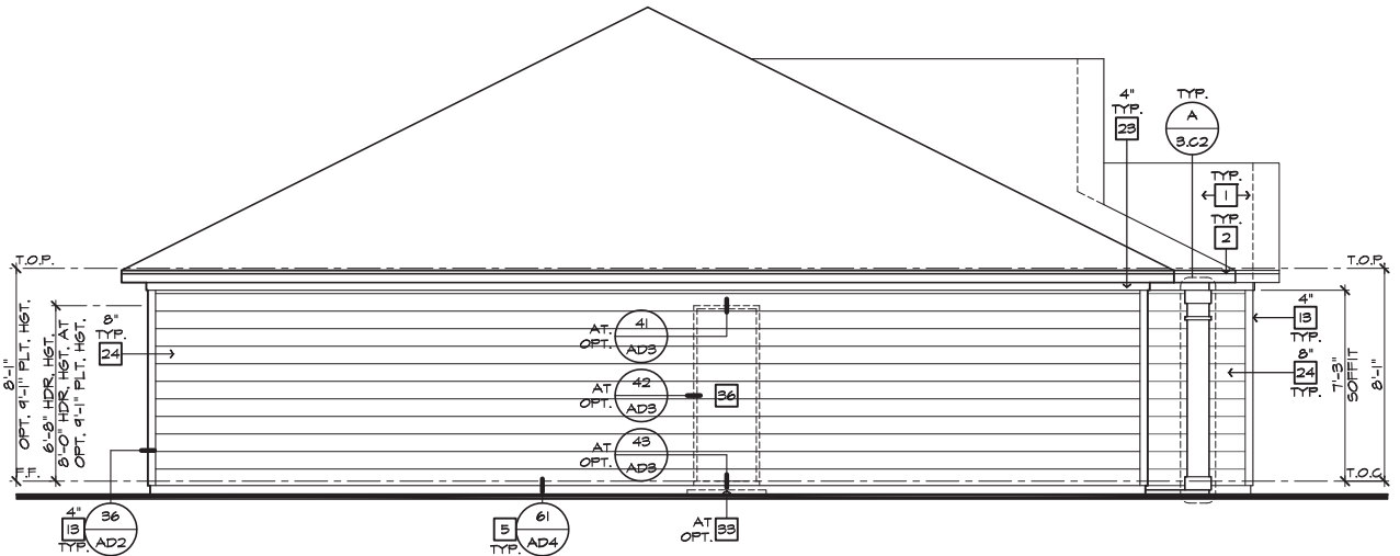
LEFT ELEVATION 'N'
