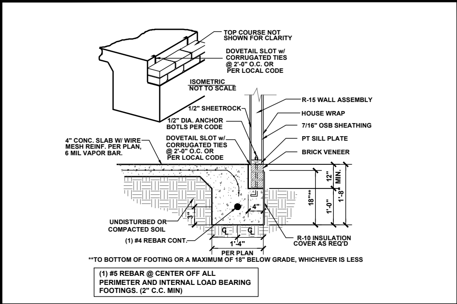
VENEER SLAB BRICK LEDGE SECTION
