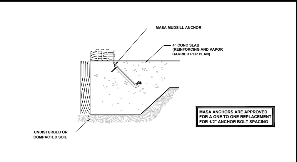
MASA FOR INSIDE OF WALL CONTINUITY
