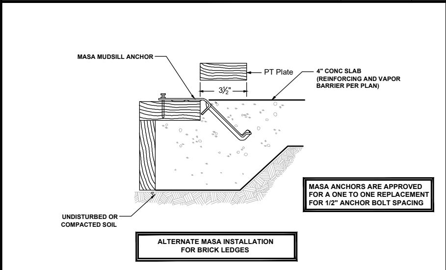
MASA FOR BRICK LEDGES
