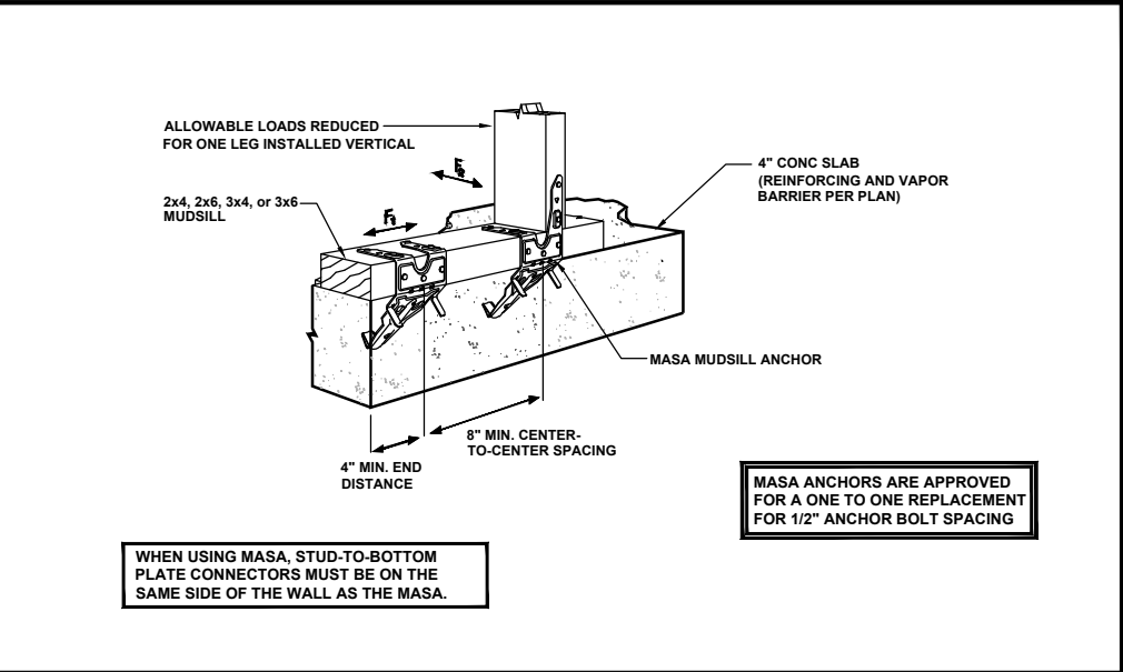
SIMPSON MASA (Z) STUD-TO-BOTTOM PLATE
