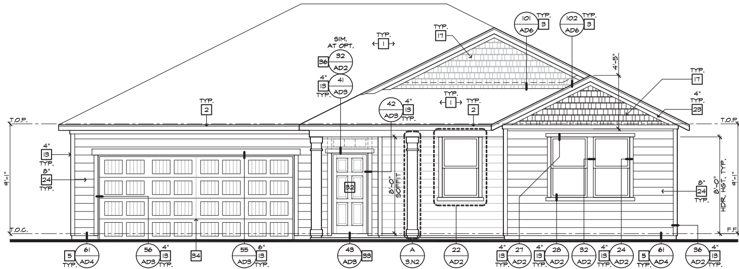
FRONT ELEVATION 'N' AT OPTIONAL 9'-1" PLT. HGT. SCALE 1/4"=1'-0" (22"X34") - 1/8"=1'-0" (11"X17")
