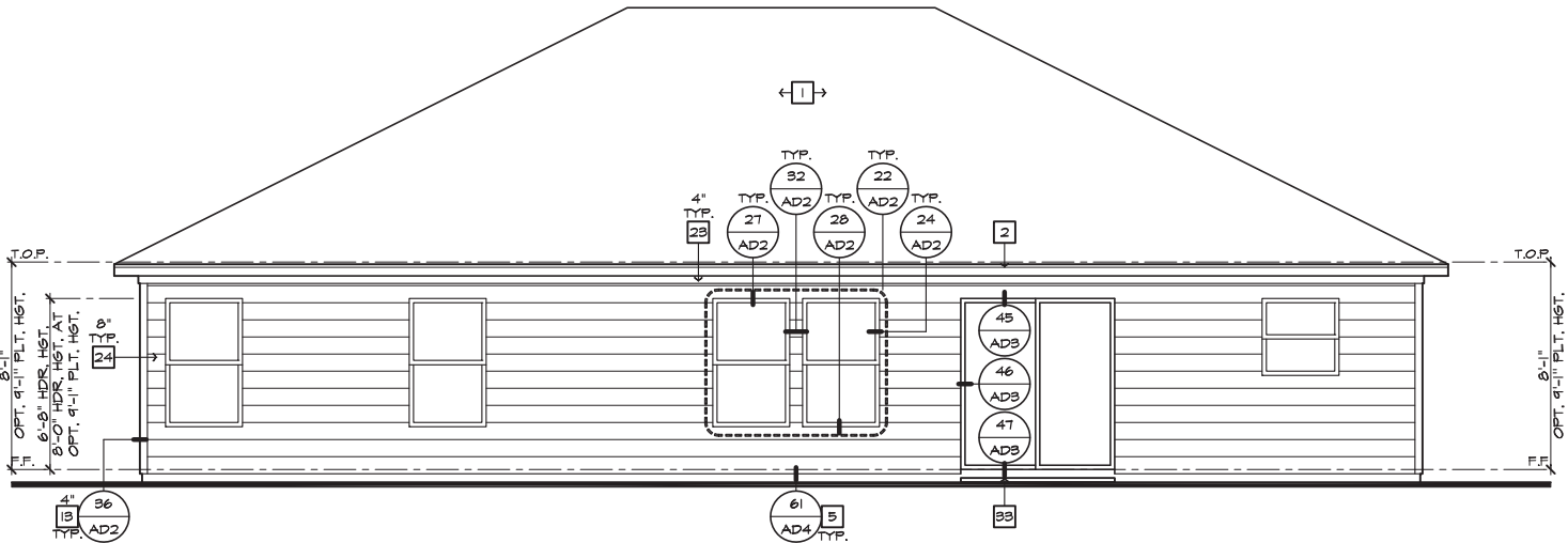
REAR ELEVATION 'N'
