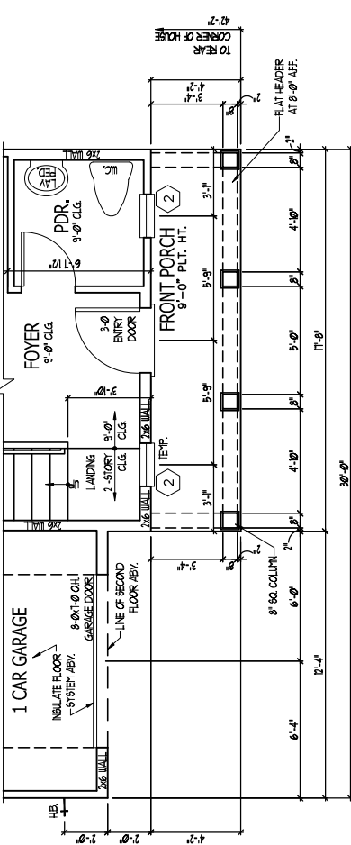
PARTIAL FIRST FLOOR B
