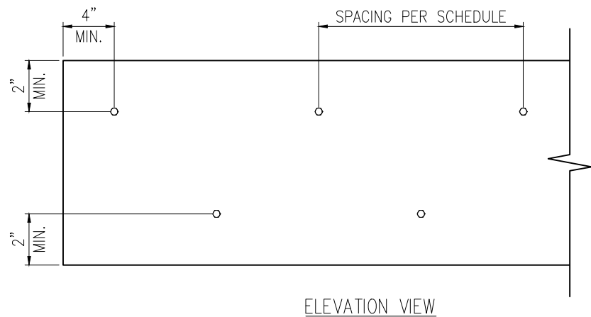
2 MULTI-PLY BEAM CONNECTION DETAIL D7f N.T.S
