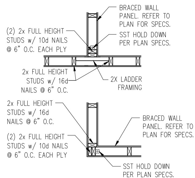
4 D9f 1" = 1'-0" TYP. HOLD DOWN DETAIL
