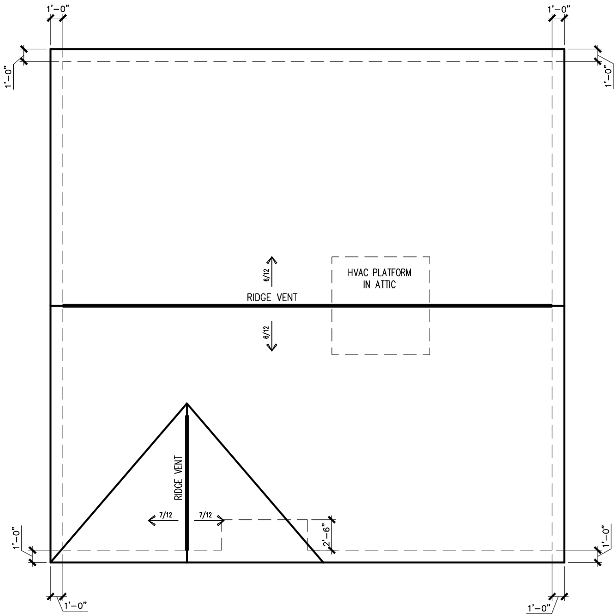
ROOF PLAN "B"
