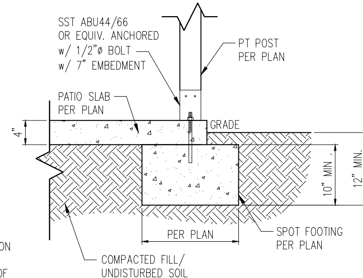
2A COVERED PATIO DETAIL D1m 3/4" = 1'-0"
