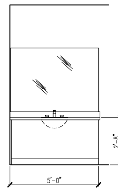
7 BATH 2
