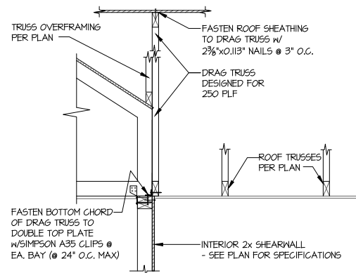
3 SHEAR TRANSFER DETAIL @ INTERIOR SHEARWALL BELOW SCALE: 3/4"=1'-0"
