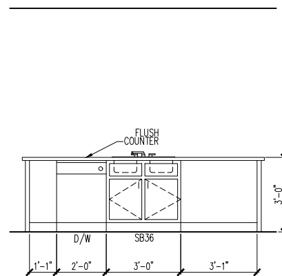
3 KITCHEN ISLAND
