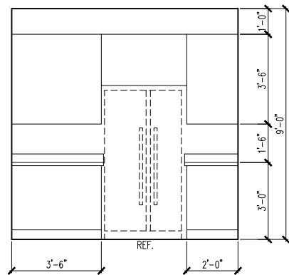
2 KITCHEN
