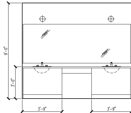
6 PRIMARY BATH
