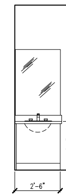
9 BATH 3
