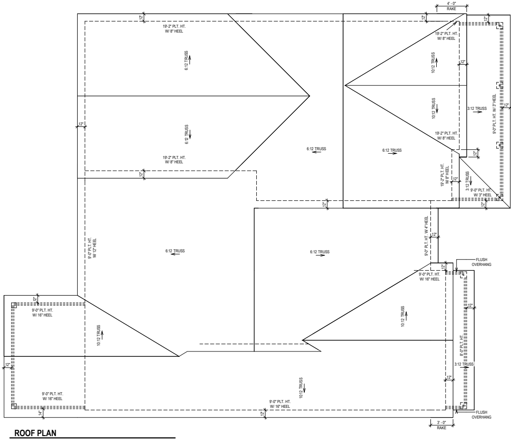
ROOF PLAN
