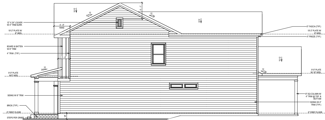
SIDE ELEVATION
