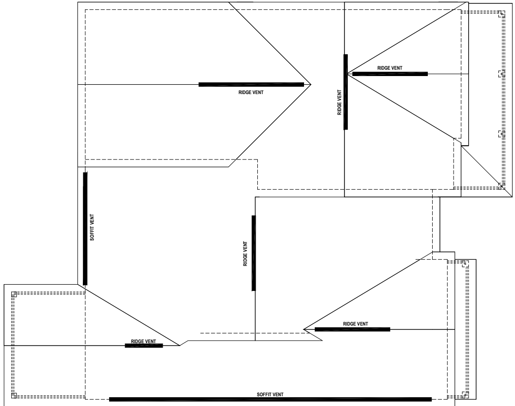
ROOF PLAN
