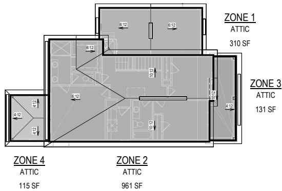
VENTILATION PLAN "B"
