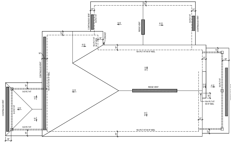
ROOF PLAN "B"
