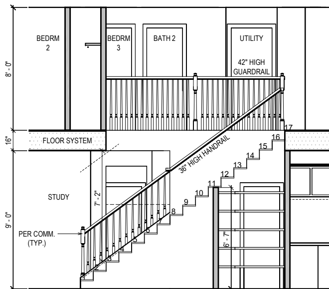
STAIR SECTION
