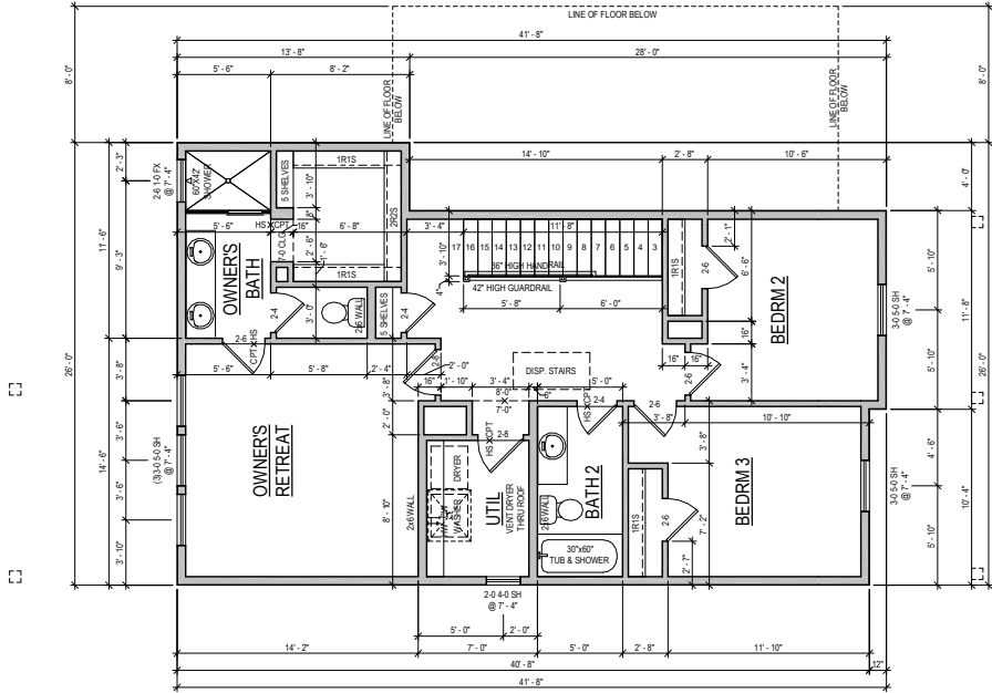
SECOND FLOOR "B"
