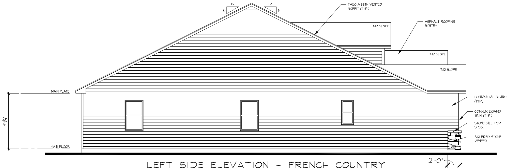
LEFT SIDE ELEVATION - FRENCH COUNTRY
