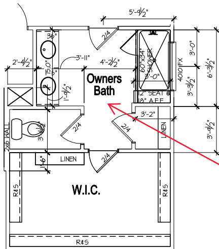
PPO - OWNER'S BATH STAND-IN SHOWER W/ SEAT
