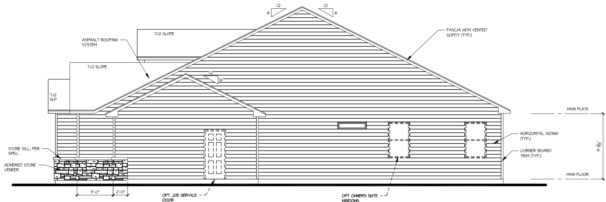
PPO - RIGHT SIDE ELEVATION - THIRD CAR GARAGE - FRENCH COUNTRY
