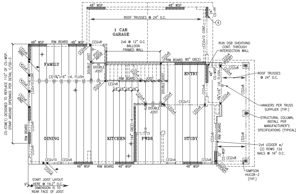
SECOND FLOOR FRAMING PLAN
