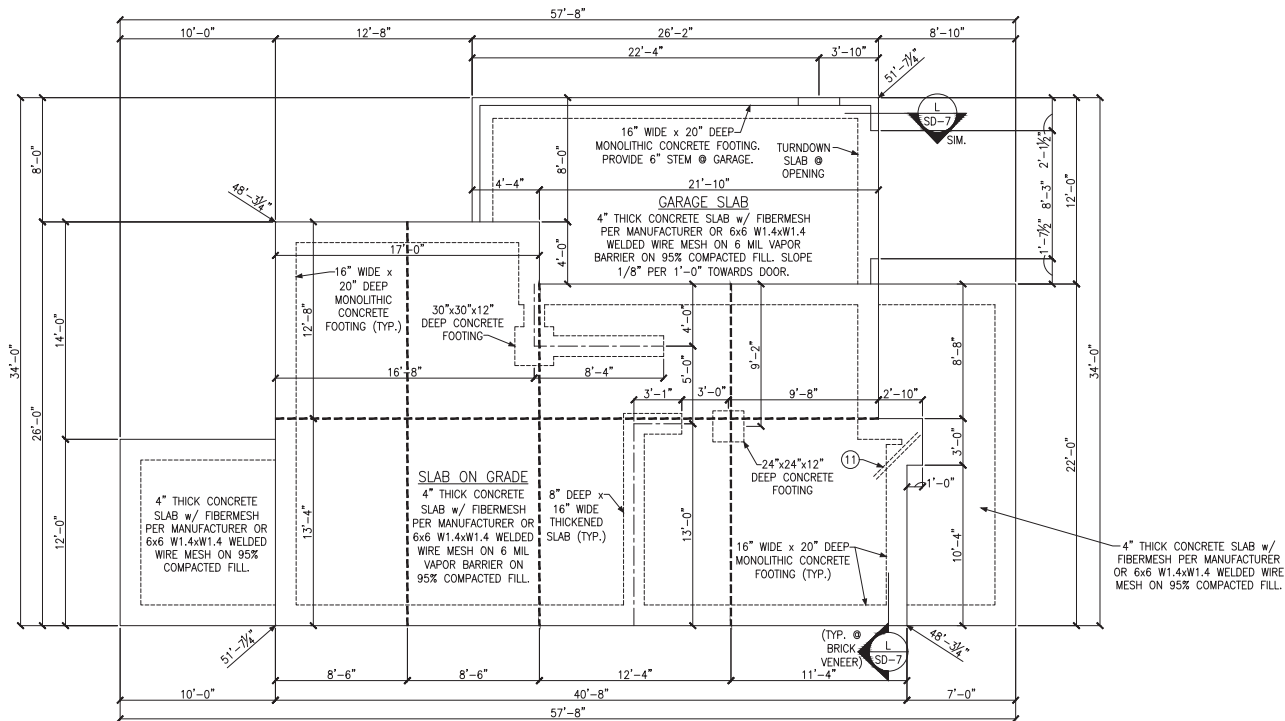
MONOLITHIC SLAB FOUNDATION PLAN
