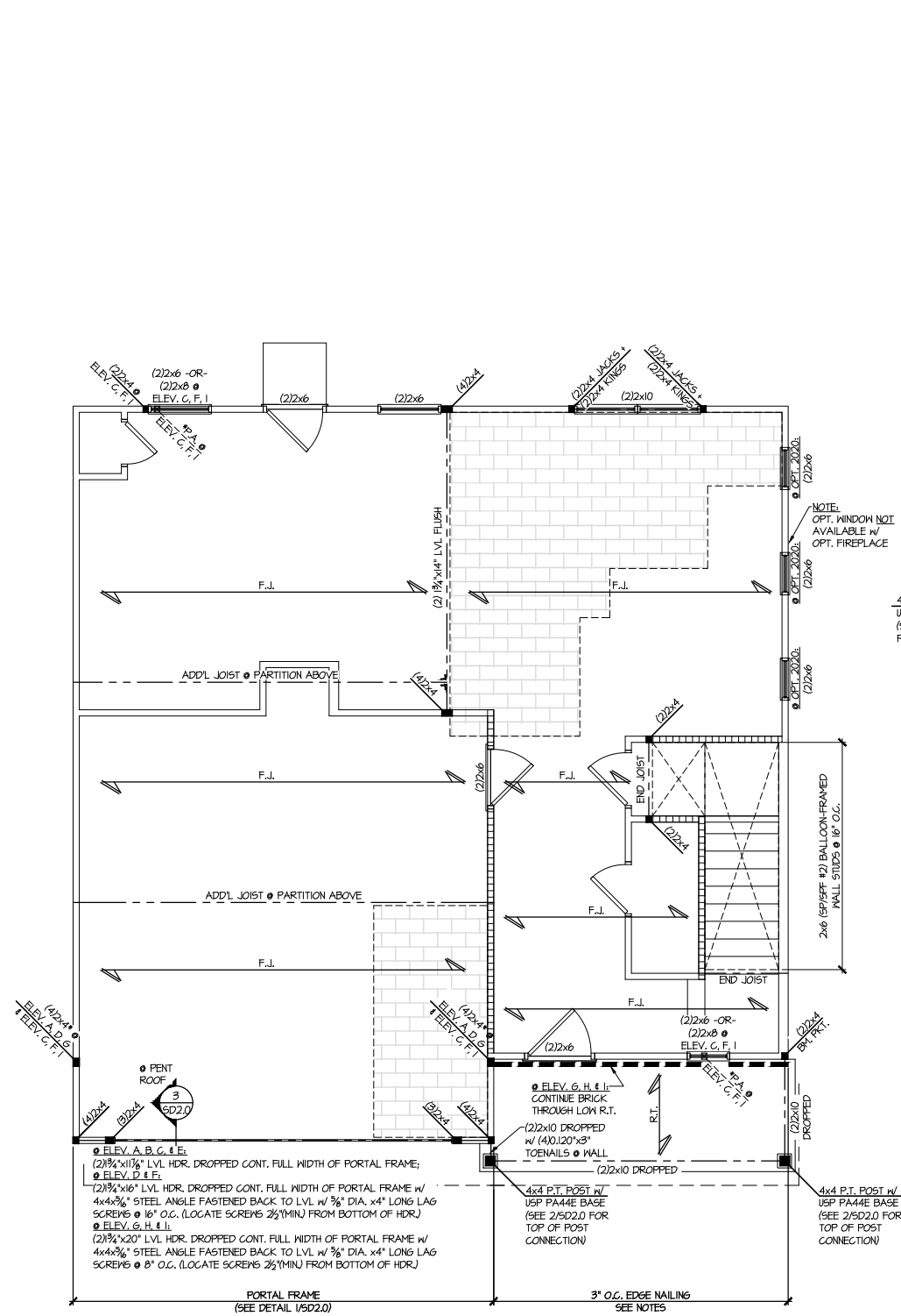
1 2ND FLOOR FRAMING PLAN SCALE: 1/4"=1'-0" ON 22x34 1/8"=1'-0" ON 11x17 ALL ELEV. SIM.
