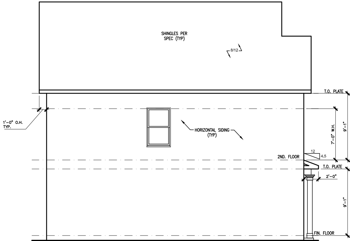
LEFT ELEVATION "B" SCALE : 1/8" = 1'-0"
