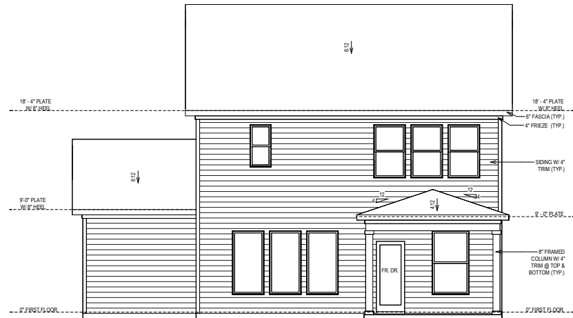
REAR ELEVATION "B"
