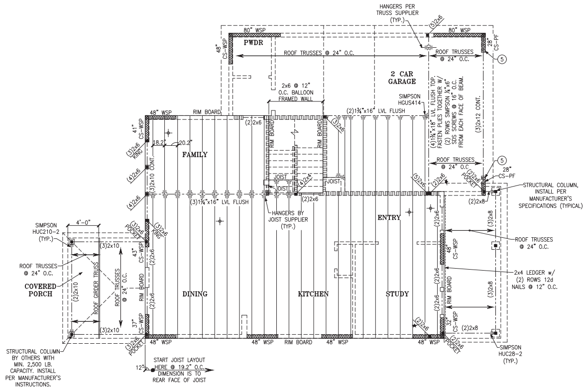
SECOND FLOOR FRAMING PLAN
